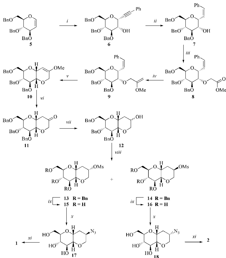
Scheme 1. Reagents and conditions: i) (a) dimethyldioxirane, acetone. (b) phenylacetylene, n BuLi, ZnCl 2 , THF, -70 °C to room temp. [6] ii) H 2 , Lindlar's catalyst, EtOAc. [6] iii) methyl bromoacetate, TBAI, NaH, DMF, 95%. iv) Cp 2 TiMe 2 , THF, 60 °C, 82%. v) dichlorido(1,3-dimesityl-2-imidazolidinylidene)(phenylmethylene)(tricyclohexylphosphane)ruthenium, CH 2 Cl 2 , reflux, 88%. vi) TFA, water, CH 2 Cl 2 , 92%. vii) L-selectride, THF, -78 °C to room temp., ( endo:exo = 2:1). viii) MsCl, Et 3 N, CH 2 Cl 2 , 0 °C, 13 40%, 14 25%, two steps. ix) H 2 , Pd/C, EtOH, 15 quant., 16 quant. x) NaN 3 , DMF, 70 °C, 17 90%, 18 94%. xi) TEMPO, NaOCl, NaHCO 3 , MeCN, 0 °C, 1 53%, 2 52%.
