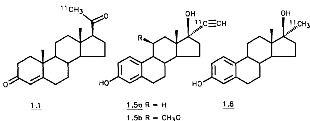
Figure 1.3 Structure of [21- 11 C]progesterone ( 1.1 ), 17α-[ 11 C]ethynylestradiol ( 1.5a ), [ 11 C]moxestrol ( 1.5b ) and 17α-[ 11 C]methylestradiol ( 1.6 ).
