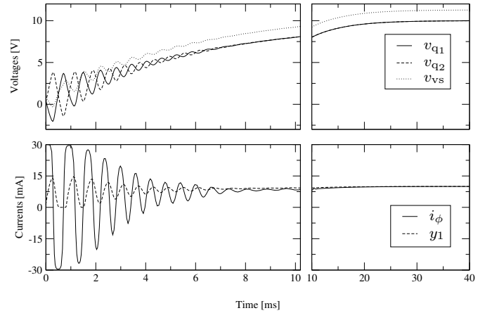
Fig. 4. Simulated response of the regulated circuit.
