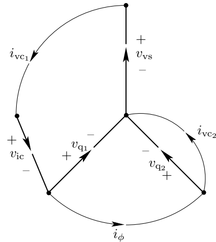
Fig. 3. Directed graph corresponding to the circuit of Figure 2. The thick straight lines represent the branches of \mathcal{T} . The thin arcs represent the links that belong to \mathcal{L} .
