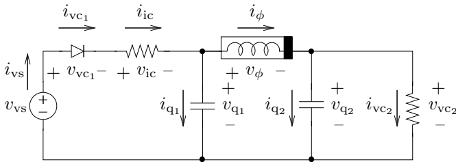
Fig. 2. An RLC circuit.
