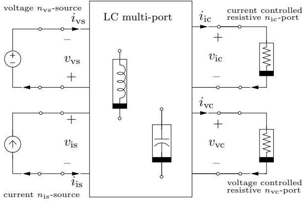
Fig. 1. An RLC network with sources and dissipation elements viewed as ports.
