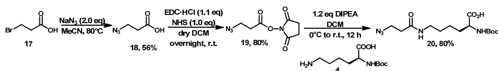
Scheme 6 Synthesis of azido lysine analogue 20
