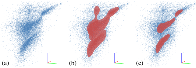
Fig. 10. CloudLasso being applied to a 3D scatter plot; data from a subset of the milliMillennium dataset [5] (showing the dimensions virial radius, R -l color, and low X-ray luminosity); (a) original 3D scatter plot, (b) initial CloudLasso selection, (c) after interactive threshold adjustment.
