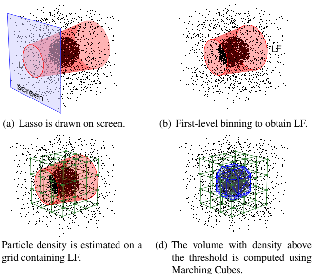
Fig. 4. Main steps of the CloudLasso selection algorithm.
