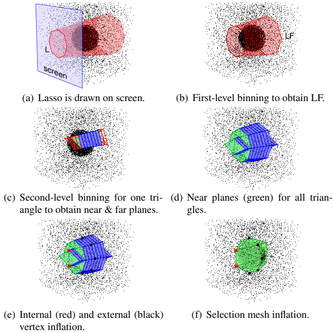
Fig. 2. Main steps of the TeddySelection algorithm.
