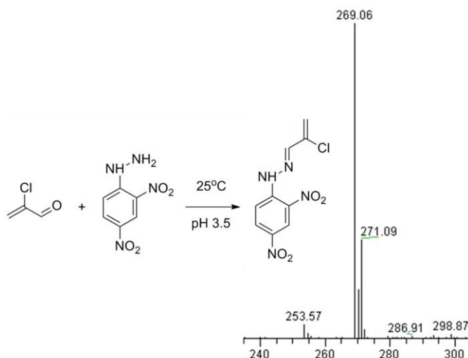
Fig. 5. Derivatization reaction of chloroacrolein with dinitrophenylhydrazine. The presence of the chloroacrolein-dinitrophenylhydrazone adduct ( m/z = 269.06 , M-H^+ ) indicates that chloroacrolein is produced.
