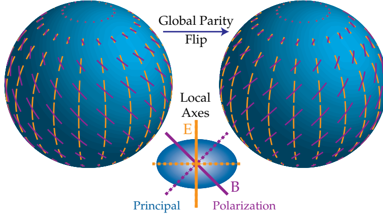
Fig. 8 The E and B polarization modes are distinguished by their behavior under parity transformation. The local distinction is that the E mode is aligned with the principle axis of polarization whereas the B mode is 45^\circ crossed with it (this figure is taken from Hu and White [86]).
