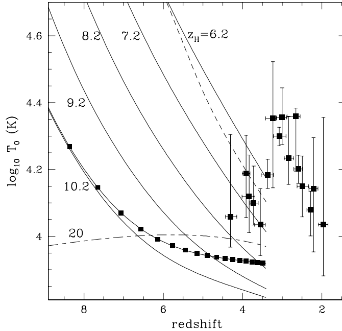
Fig. 11 Temperature evolution of the IGM above redshift 3.4. The solid curves indicate the evolution of the temperature at the mean density for various H I reionization redshifts z_H , as indicated. The temperature after hydrogen reionization is assumed to be T_0 = 6 \times 10^4 \text{K} , and the hydrogen photoionization rate is \Gamma = 10^{-13} \text{s}^{-1} ( \Gamma = 10^{-14} \text{s}^{-1} , short-dashed curve). The He II photoionization rate is adjusted so that the He III abundance is x_{\text{HeIII}} \approx 0.1 at z = 3.5 . The solid curve connecting the filled squares indicates z_H = 10.2 and a higher He II photoionization rate, x_{\text{HeIII}}(z = 3.5) = 0.6 . Finally, the long-dashed curves has z_H = 20 but a still higher He II photoionization rate, x_{\text{HeIII}}(z = 3.5) = 0.95 . If He is mostly singly ionized at z \approx 3.5 , then the rapid decrease in T_0 after reionization places an upper limit of z_H < 9 on the redshift of hydrogen reionization. The filled squares with error bars show the measured IGM temperature as a function of redshift. This figure taken from [202].
