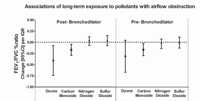
Figure 2: Ambient air pollution is associated with airflow obstruction
