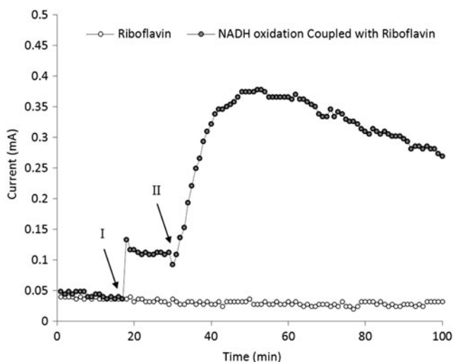
FIG. 5. Current production in a fuel cell due to oxidation of NADH ( E^{\circ} = -0.32\text{ V} ) coupled to the electrochemical oxidation of riboflavin ( E^{\circ} = -0.21\text{ V} ) with concomitant electrochemical reduction of potassium ferricyanide ( E^{\circ} = 0.36\text{ V} ). (I) When 1 mM NADH was introduced into the anode chamber, a current was generated due to direct oxidation of NADH. (II) When 200 \mu\text{M} of riboflavin was introduced into the anode compartment, the current increased several fold due to oxidation of NADH mediated by riboflavin ( \bullet — \bullet ). Current was not produced when 200 \mu\text{M} riboflavin was introduced into the anode chamber alone ( \circ — \circ ).
