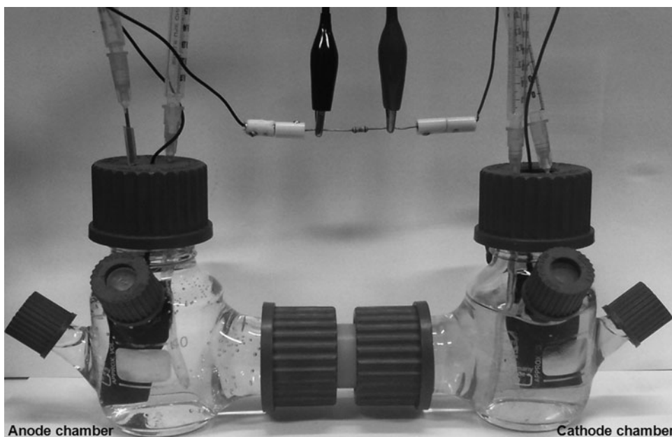
FIG. 1. Microbial fuel cell employed in the present studies.
