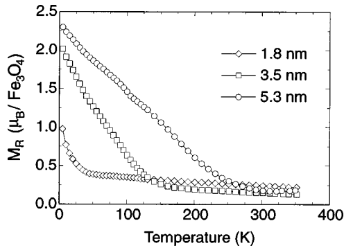
FIG. 3. Remanent magnetization M_R , in units of \mu_B per formula unit \text{Fe}_3\text{O}_4 , of \text{Fe}_3\text{O}_4/\text{MgO} multilayers, after saturation in an external field of 1 T at 5 K, as a function of temperature and \text{Fe}_3\text{O}_4 layer thickness.
