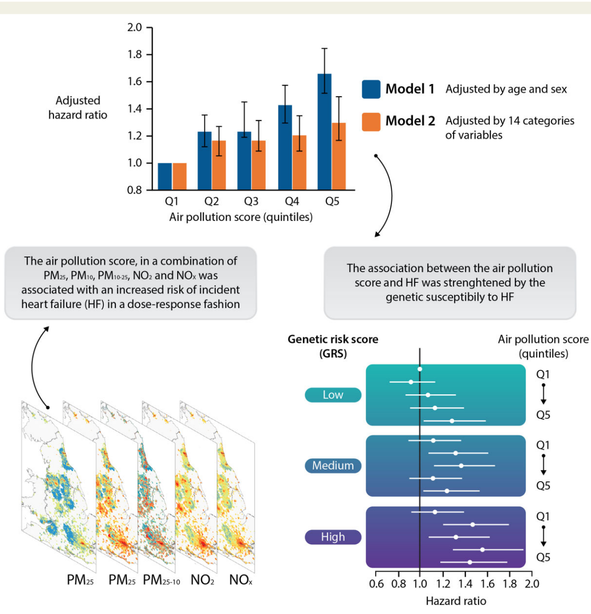
Figure 2 Long-term joint exposure to various air pollutants, including PM2.5, PM10, PM2.5–10, NO2, and NOx is associated with an elevated risk of incident heart failure in an additive manner. Persons with genetic higher susceptibility to heart failure displayed a particularly high risk of heart failure. Reprinted with permission from Wang et al. 6
