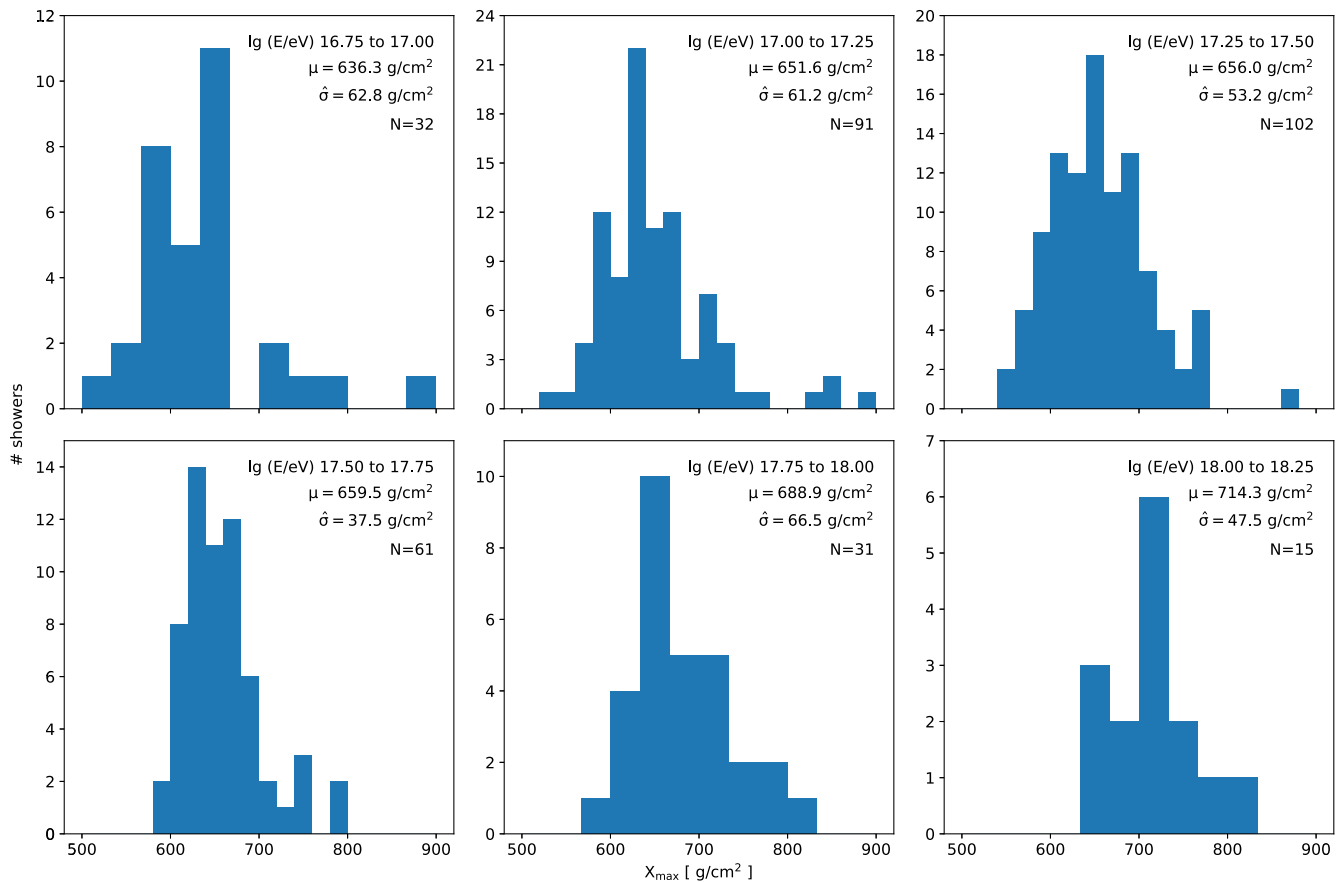
FIG. 7. Histograms of X_{\max} for each energy bin. The average ( \mu ) and standard deviation estimates ( \hat{\sigma} ) per bin are as shown in Figs. 4 and 6, respectively.
