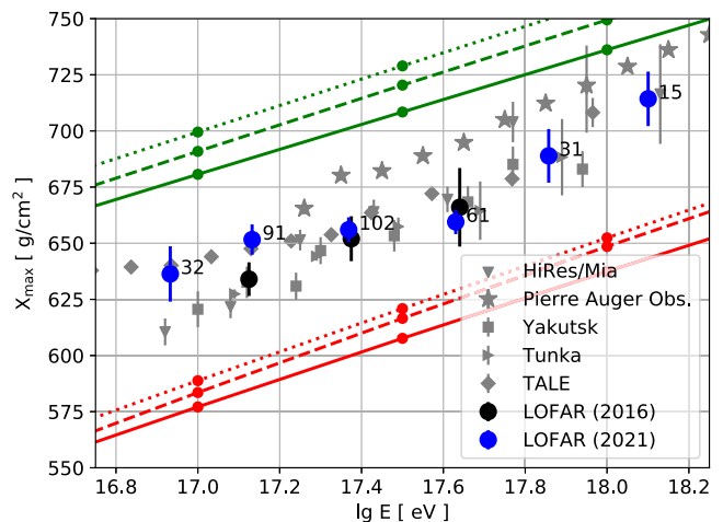
FIG. 4. The average depth of shower maximum X_{\max} , as a function of primary particle energy. The annotated numbers indicate the number of showers in each bin, and the error margins indicate the uncertainty on the mean of the X_{\max} distribution. The upper lines indicate the mean values expected for protons, from simulations with QGSJetII-04 (solid), EPOS-LHC (dashed) and Sibyll-2.3d (dotted). The lower lines show the mean predicted values for iron nuclei. For comparison, results from Pierre Auger [39], Yakutsk [40], Tunka [41], HiRes/Mia [42], and TALE [43] are included.
