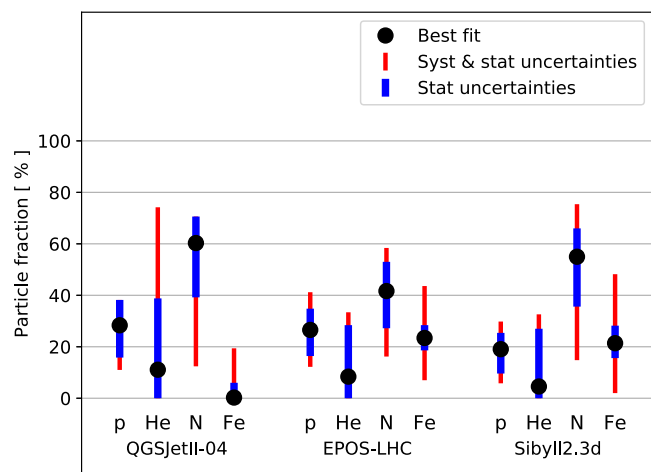
FIG. 12. Composition results from our dataset, assuming each of the three hadronic interaction models shown at the bottom. The best fit is shown along with statistical and systematic uncertainties.
