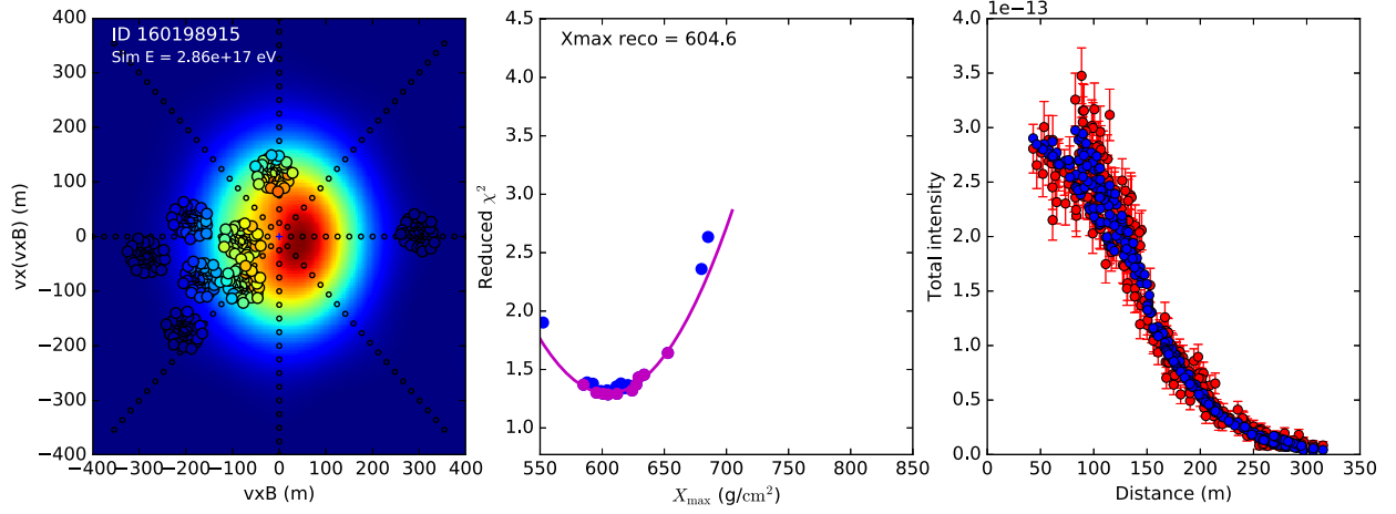
FIG. 1. An example of fitted CoREAS showers to a LOFAR-measured shower. The left panel shows simulated signal energy along with the measurements, in the shower plane, for the best-fitting shower. The lateral intensity (and pulse energy) distribution is not rotationally symmetric. The middle panel shows the reduced \chi^2 as a function of X_{\max} , with a parabolic fit through the lower envelope denoted by the magenta line. The right panel shows a 1D lateral distribution function, where red points with uncertainties denote the measurements, and blue points denote the simulated intensities.
