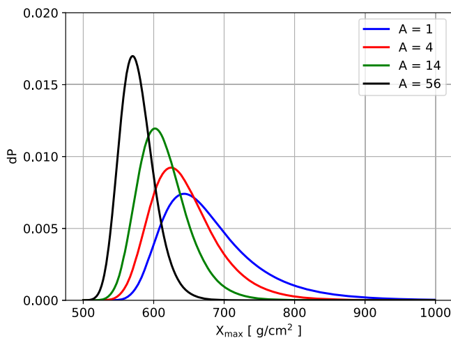
FIG. 3. The probability density functions for the depth of shower maximum X_{\max} , for the elements H, He, N, and Fe, at energy 10^{17} \text{ eV} and hadronic interaction model QGSJetII-04.
