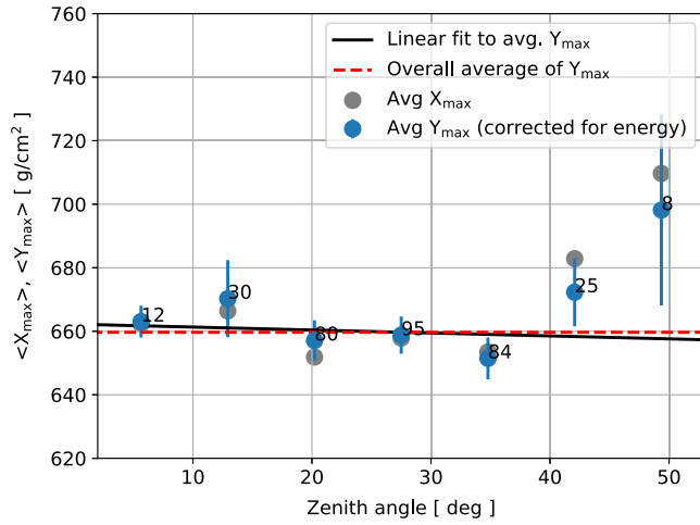
FIG. 8. Average Y [from Eq. (6)] versus zenith angle, together with a constant and linear fit.
