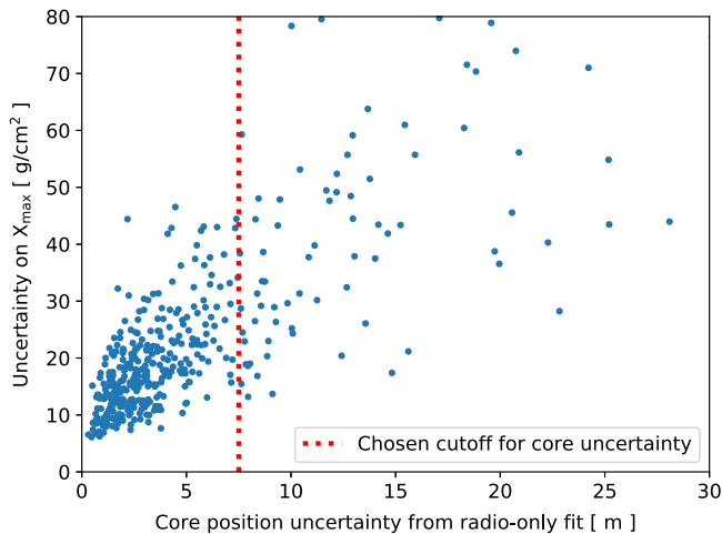
FIG. 2. The uncertainty on X_{\max} versus the uncertainty on the core position, per measured shower, after cuts on energy and fiducial selection criteria. The dotted line indicates the chosen cutoff.
