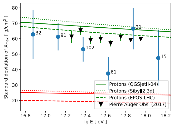
FIG. 6. The standard deviation of X_{\max} as a function of primary particle energy. The margins indicate the uncertainty on the standard deviation of the X_{\max} distribution. Results from the Pierre Auger Observatory are shown, together with the values from simulations of protons and iron nuclei (high and low lines, respectively).
