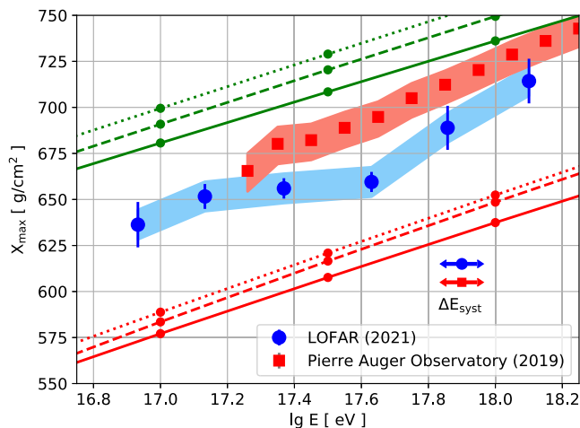
FIG. 5. Average X_{\max} versus primary energy, for LOFAR and Pierre Auger Observatory, with colored bands indicating their systematic uncertainty on X_{\max} . The uncertainty margins per data point are statistical uncertainties only. The systematic uncertainty on energy is the same for both experiments and is indicated by the arrows to the lower right.
