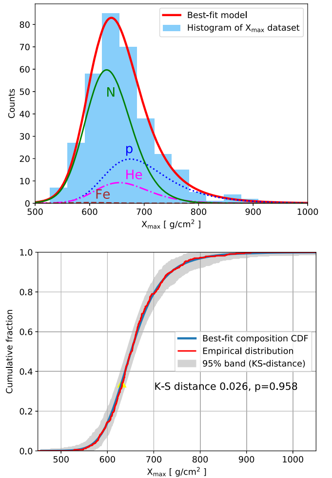
FIG. 10. Top: A histogram of X_{\max} , together with the best-fitting distribution from Eq. (3). Bottom: The cumulative distribution corresponding to the best-fit composition model, together with the empirical distribution from our dataset. The yellow arrow indicates where the distance between CDF and empirical distribution is maximal. The grey band is the envelope of all simulated empirical distributions that have a K-S distance to the CDF below its 95-percentile level. Both graphs indicate a good fit.
