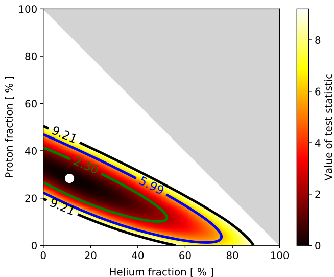
FIG. 11. Contour plot of the proton and helium fraction, giving the regions consistent with a one-sigma, 95% and 99% confidence level, respectively.
