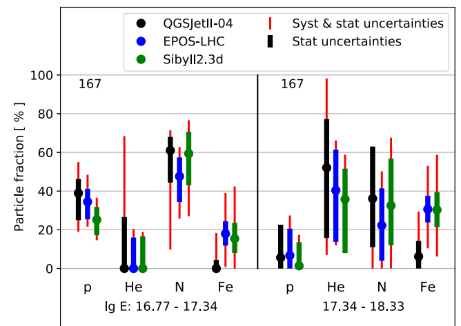
FIG. 13. Mass composition results in two energy bins. The energy ranges per bin are shown; their main coverage is at 17.14 \pm 0.13 , and 17.65 \pm 0.23 , respectively.
