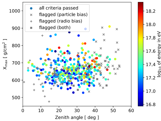
FIG. 9. Scatter plot of X_{\max} versus zenith angle, for all 469 showers with core reconstruction precision better than 7.5 m. Colored circles represent the 334 showers passing all criteria, with the color denoting their energy. The showers flagged by the particle and radio bias tests are also shown.
