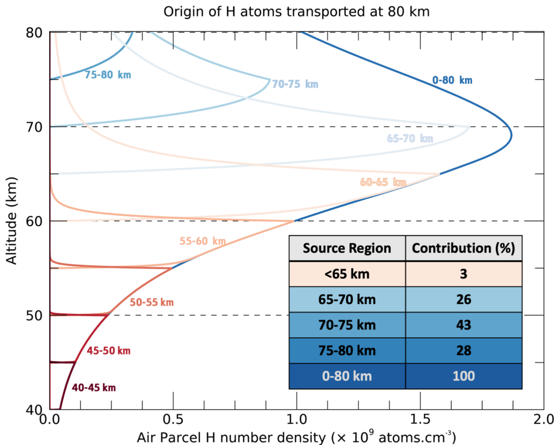
Figure 5: Air parcel model predictions for a set of configurations where production only occurs in a 5 km-thick layer whose top altitude we vary from 45 to 80 km. Plotted quantity is the H number density ( \text{atoms.cm}^{-3} ) in the parcel. The shape of each curve reflects the processes at work inside the parcel during its ascent at 10 cm/s. Below 55 km, H is instantaneously lost after leaving its production zone. Then, its increasing lifetime allows it to ascend several km before destruction. Above 60 km, an increasing fraction of the produced atoms can be advected up to 80 km. The contribution of each 5 km layer is calculated by dividing their corresponding N_H at 80 km with that of the 0-80 km case, that is the nominal full production case.
