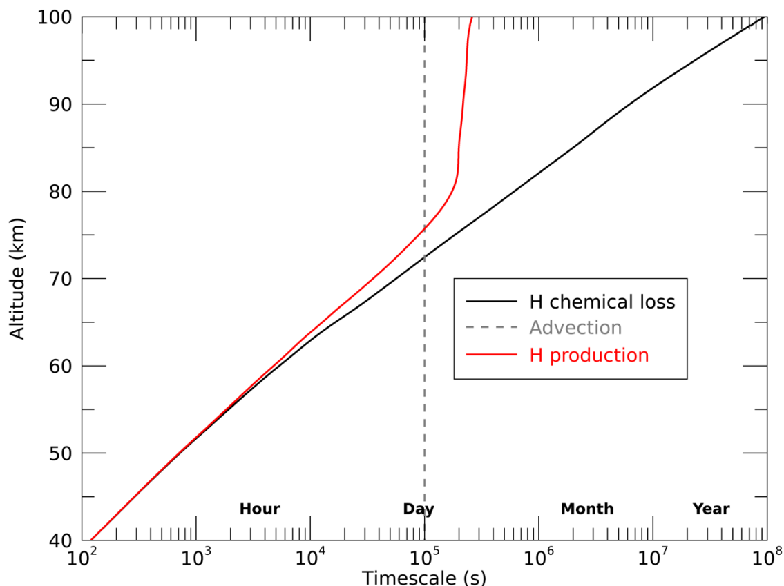
Figure 4: Timescales associated with the various processes represented in the air parcel model, transport timescale is deduced from an ascent velocity of 10 cm/s.
