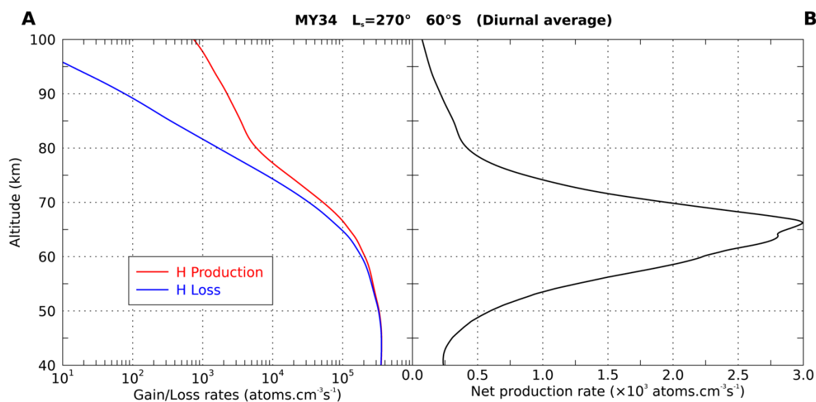
Figure 3: (A) H production and loss rates as predicted by a photochemical model for the MY34 Perihelion case, using pressure, temperature, and water vapor profiles obtained by ACS MIR channel. H production is only due to water vapor photolysis. H loss relies on reactions with O_3 , HO_2 , and O_2 . (B) H net budget calculated by subtracting loss from production rates.
