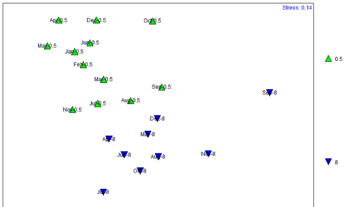
Fig. 4: NMDS ordination based on the epilithic diatom relative abundance (%) data in the shallow ( \blacktriangle - 0.5 m) and deep ( \blacktriangledown - 8 m) sites in Neum Bay in 2011.
