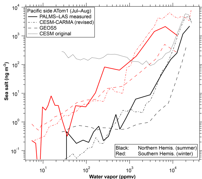
Figure 7. Model correlations for the CESH-CARMA and GEOS-5 models. ATom2 and tropical curves are omitted for simplicity. GEOS-5 model output was sampled along the flight tracks and CESH-CARMA at all altitudes in a curtain along the flight tracks. Also shown is one curve from the CESH-CARMA model before a revised convective aerosol removal scheme was implemented (Yu et al., 2019).
