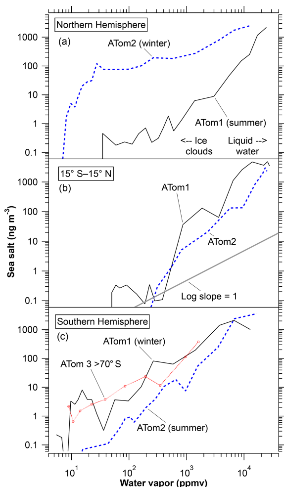
Figure 6. Measured average sea-salt mass concentrations as a function of water vapor. Latitude bands for the Northern and Southern hemispheres are 20 to 65° except for the labeled data over Antarctica. All data except those beyond 70° S are from the Pacific Ocean side of North and South America. Arrows in panel (a) show approximate water mixing ratios above which most clouds are liquid water and below which most clouds are ice. One way to view the graph is to consider water vapor as a vertical scale with wet air at low altitudes and dry air at high altitudes. In both hemispheres the winter data show more sea-salt aerosol in the upper troposphere at a given amount of water vapor than either the summer hemisphere or the tropics.
