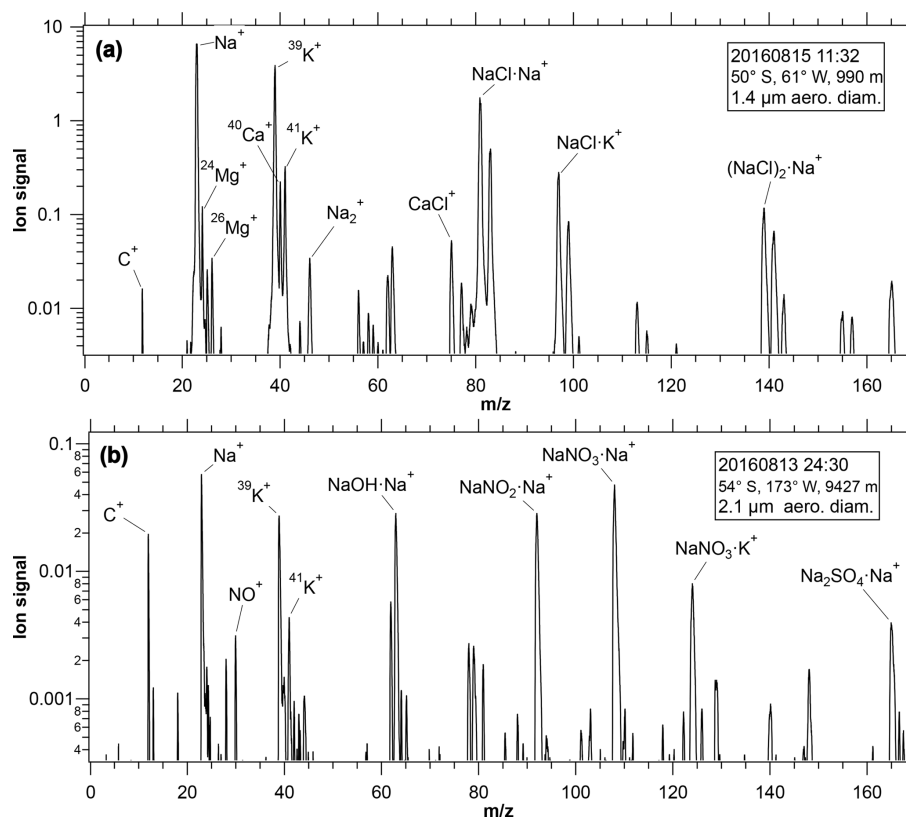
Figure 1. Mass spectra of (a) a typical sea-salt particle and (b) a highly processed sea-salt particle where the chloride has been replaced by nitrate and sulfate. The spectrum in panel (a) is chosen to be similar to the average of all low-altitude spectra of sea salt.
