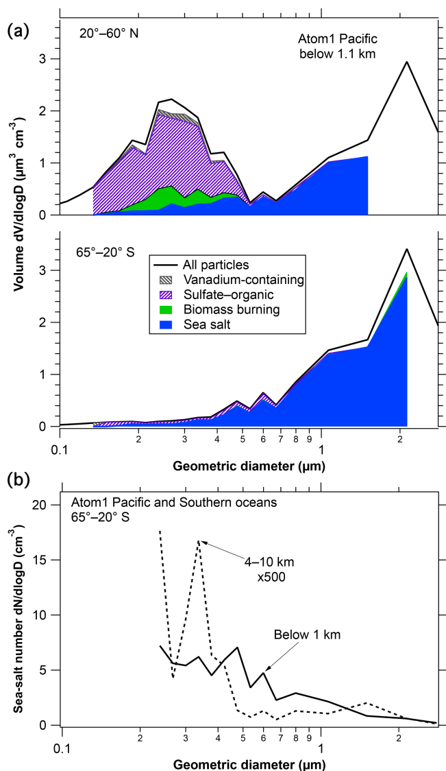
Figure 4. Size distributions of sea-salt particles in the marine boundary layer. Panel (a) shows how the total size distribution (black line) is multiplied by PALMS composition at each size to obtain the volume of sea-salt particles. White areas below the size distribution curves represent unknown compositions or, at the largest and smallest diameters, insufficient data to assign composition. The reduced concentration above about 3\ \mu\text{m} diameter is because the aircraft inlet does not efficiently transmit larger particles. Panel (b) compares the number size distributions at low and high altitudes.
