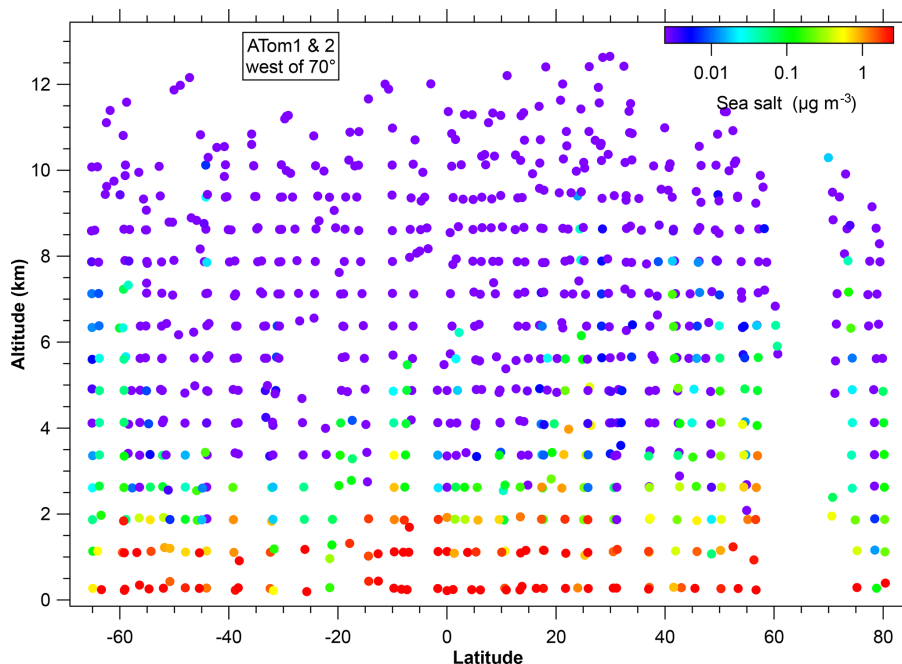
Figure 3. Concentration of sea-salt aerosol during the ATom1 and ATom2 flights over the Arctic, Pacific, and Southern oceans. The blank region between about 60 to 70° N is because of flying over land (Alaska). The color scale is from 2.5 \text{ ng m}^{-3} to 2.5 \text{ } \mu\text{g m}^{-3} (at standard conditions). These concentrations include sea-salt particles between about 180 nm and 3 \text{ } \mu\text{m} diameter. Data are averaged over bins of 750 m vertically and about 4^\circ latitude; points are plotted at the midpoint location of the data within each bin.
