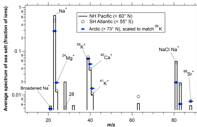
Figure 5. Average spectra of sea-salt particles larger than 1\ \mu\text{m} diameter for the Arctic and lower latitude regions during ATom2. Na peaks were smaller over the Arctic Ocean than over the Pacific Ocean in the Northern Hemisphere. The South Atlantic is included to provide an estimate of consistency between regions that should be similar. Spectra were selected that have ion intensities large enough to measure minor peaks but that will not significantly saturate the Na peak. n \approx 5500 for the NH Pacific, 700 for the SH Atlantic, and 300 for the Arctic.
