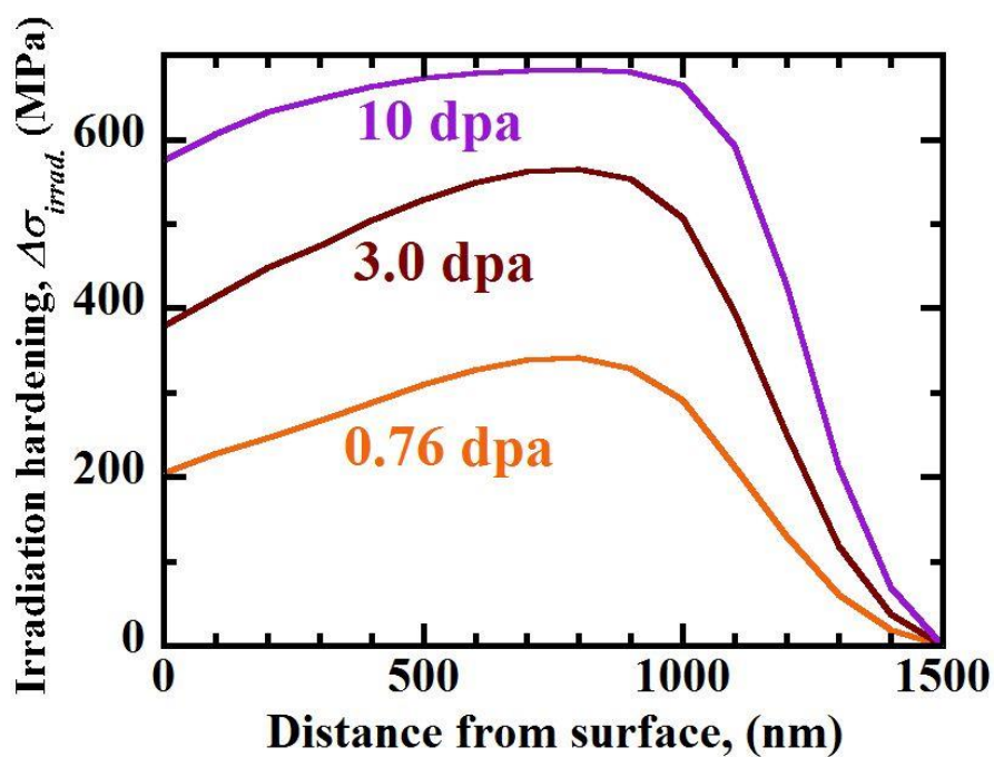
Fig. 8. Depth profiles of irradiation hardening determined by a combination between Makin-Minter model and SRIM calculation.
