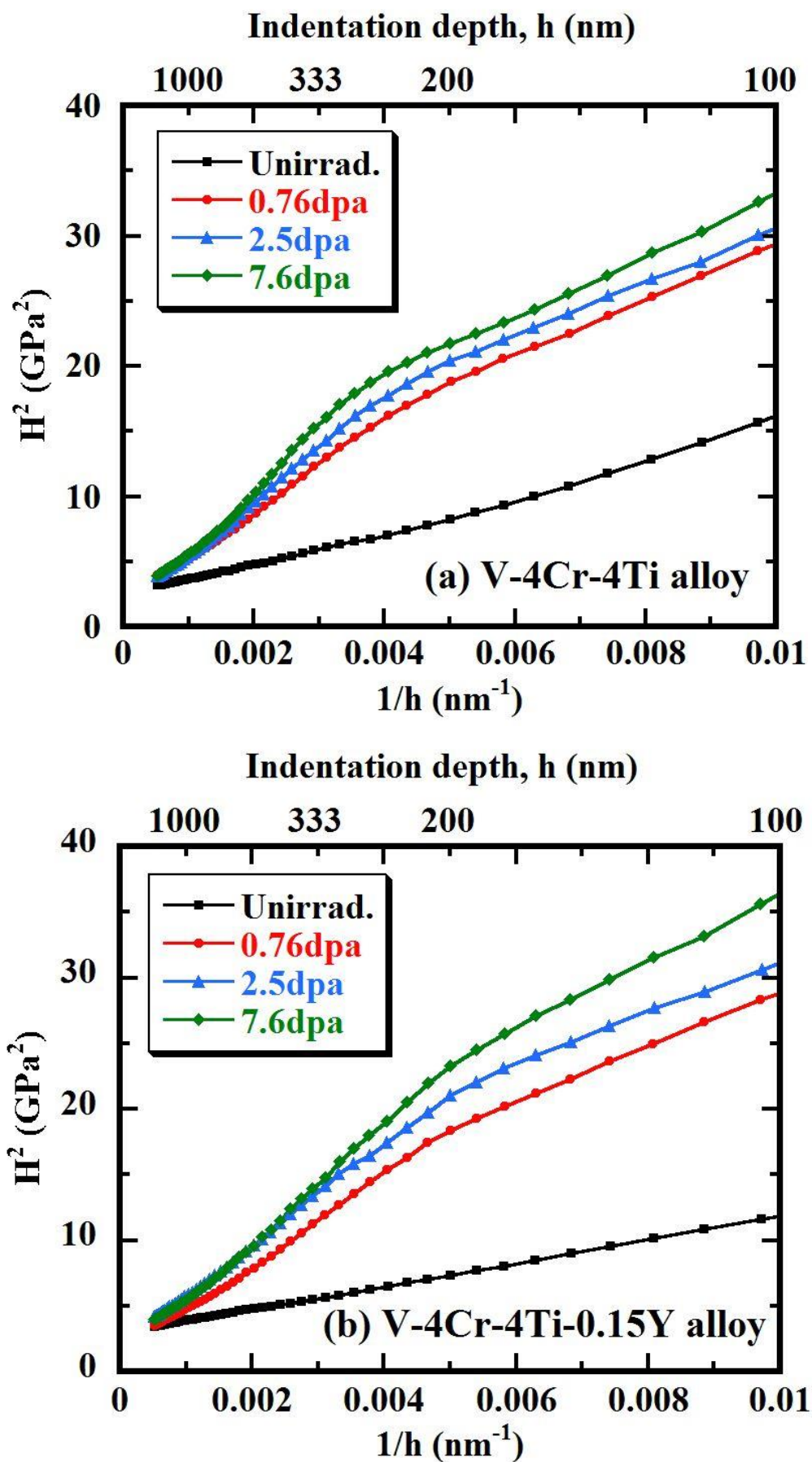
Fig. 4. Plots of H^2 versus 1/h for (a) V-4Cr-4Ti alloy and (b) V-4Cr-4Ti-0.15Y alloy.
