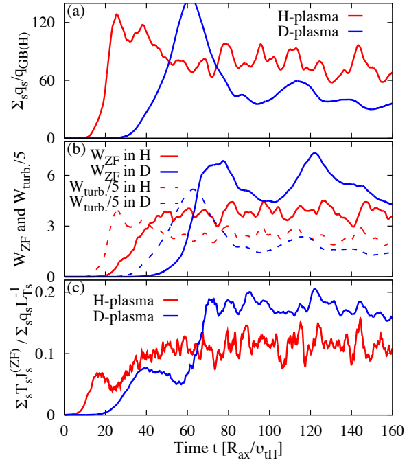
FIG. 2: Impacts of the hydrogen isotope mass on (a) turbulent heat fluxes normalized by the hydrogen gyro-Bohm unit ( \sum_s q_s / q_{GB(H)} ), (b) turbulence ( W_{turb.} ) and zonal-flow ( W_{ZF} ) energy, and (c) normalized entropy transfer to zonal flows ( \sum_s T_s \mathcal{T}_s^{(ZF)} / \sum_s q_s L_{T_s}^{-1} ), where s = \{i, e\} , and \nu_{ei}^* = 0.07 .
