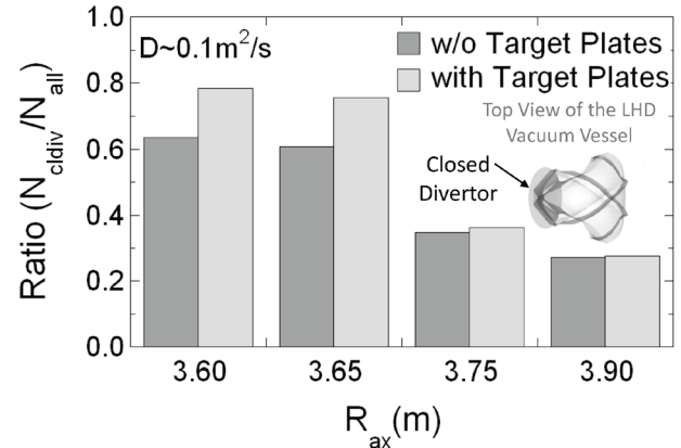
Fig. 3. Histograms of the ratio of the number of the strike points locating in the closed divertor region on that of all strike points. The ratios in the case with and without the target plates are indicated in the four magnetic configurations ( R_{ax}=3.60\text{m}\sim 3.90\text{m} ).
