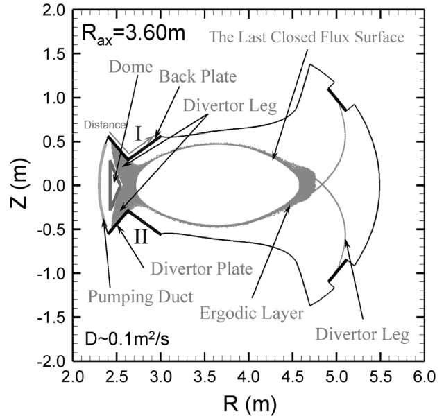
Fig. 5. Poincare plot of the magnetic field lines in the plasma periphery for R_{ax}=3.60\text{m} with the poloidal cross section of the closed divertor components. The plot includes the effect of the particle diffusion ( D \sim 0.1\text{m}^2/\text{s} ).
