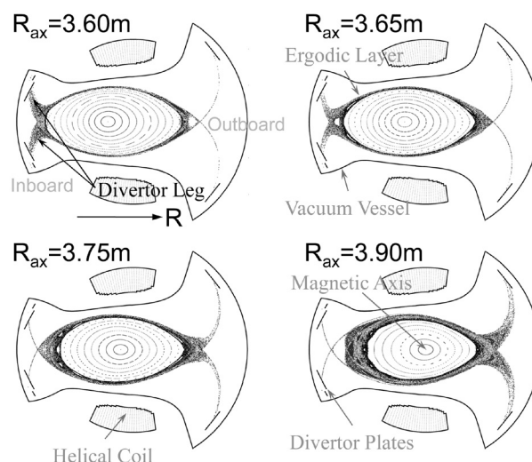
Fig. 1. Poincaré plot of the magnetic field lines in magnetic surfaces, the ergodic layer and the divertor legs in four different magnetic configurations in LHD ( R_{ax}=3.60\sim 3.90m ).
