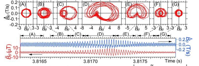
FIG. 6 Trajectories in phase space ( \dot{B}_\theta - \tilde{B}_\theta space). \dot{B}_\theta and \tilde{B}_\theta associated with the secondary mode and primary mode are extracted by numerical filters with the pass bands of 25 – 55 kHz and 58 – 92 kHz, as shown in the bottom panel.
