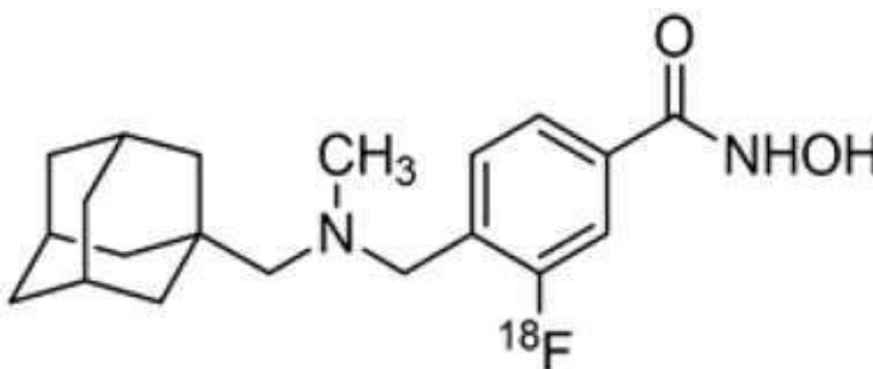
Figure 1- [ 18 F]EKZ-001 Structure [9] 1
