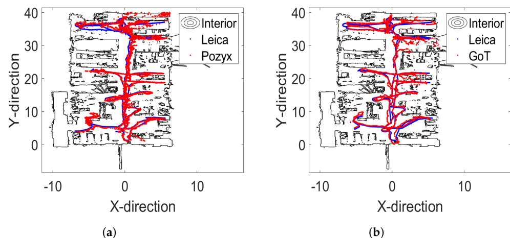
Figure 13. Two-dimensional traces for dynamic trajectory. (a) Laboratory outline (ROSmapping) and Leica (blue)/Pozyx (red) traces. (b) Laboratory outline (ROSmapping) and Leica (blue)/GoT (red) traces.
