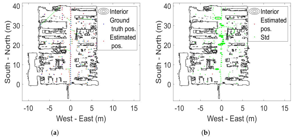
Figure 4. Static case results for GoT at 1m altitude. (a) Estimated positions from GoT (red) vs. ground-truth (blue) with connecting line (green). (b) Estimated positions from GoT (red) and standard deviation ellipsoids (green).
