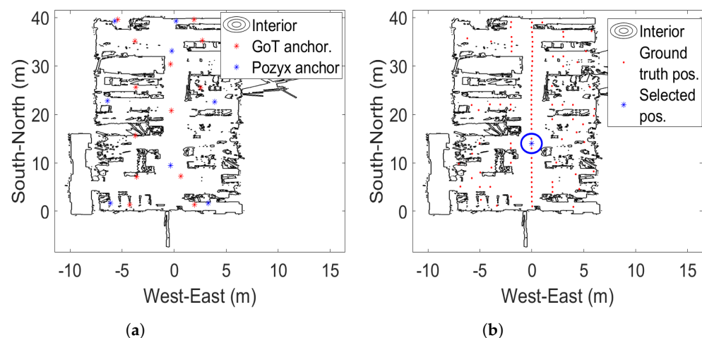
Figure 2. (a) Laboratory outline (ROsmap). Placement of Pozyx (blue) and GoT (red) anchors. (b) Placement of 100 ground-truth reference points (red). Ground truth point selected for detailed analysis (in blue circle).
