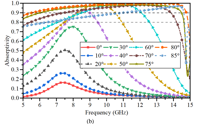
Fig. 6 Simulated absorptivity at different incident angles in in two polarization planes (a) \varphi = 0^\circ , (b) \varphi = 90^\circ .
