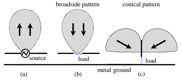
Fig. 1 (a) Radiation and (b) absorption patterns of a horizontal dipole antenna, and (c) absorption pattern of a vertical monopole antenna.
