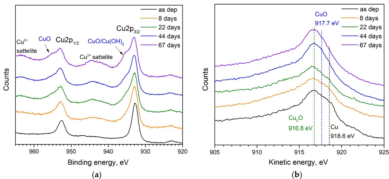
Figure 3. Time evolution of (a) XPS and (b) AES spectra of Cu NPs kept in ambient conditions. Characteristic peaks related to \text{Cu}2p_{3/2} and \text{Cu}2p_{1/2} states, \text{Cu}^{2+} satellites as well as bands related to \text{Cu}(\text{OH})_2 and \text{Cu}(\text{II}) oxide are indicated in panel (a). Vertical dashed lines in panel (b) show the energies for \text{Cu}(\text{I}) and \text{Cu}(\text{II}) oxides as well as for metallic Cu.
