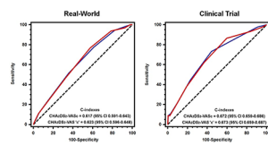
Fig. 2 Receiver operating characteristic curves of CHA 2 DS 2 -VASc vs. CHA 2 DS 2 -VASc'c' scores in Real-World and Clinical Trial. Blue line = CHA 2 DS 2 -VASc; Red line = CHA 2 DS 2 -VASc'c'. C-index comparison: Real-World (p = 0.312); Clinical Trial (p = 0.954)
