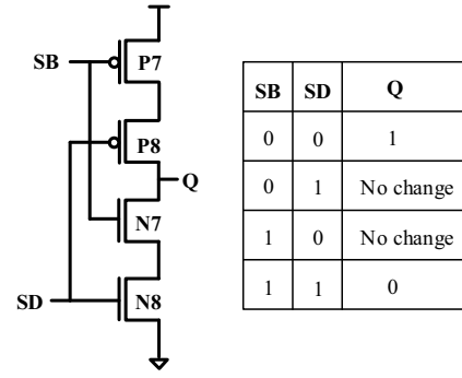
FIGURE 8 Muller C-element
