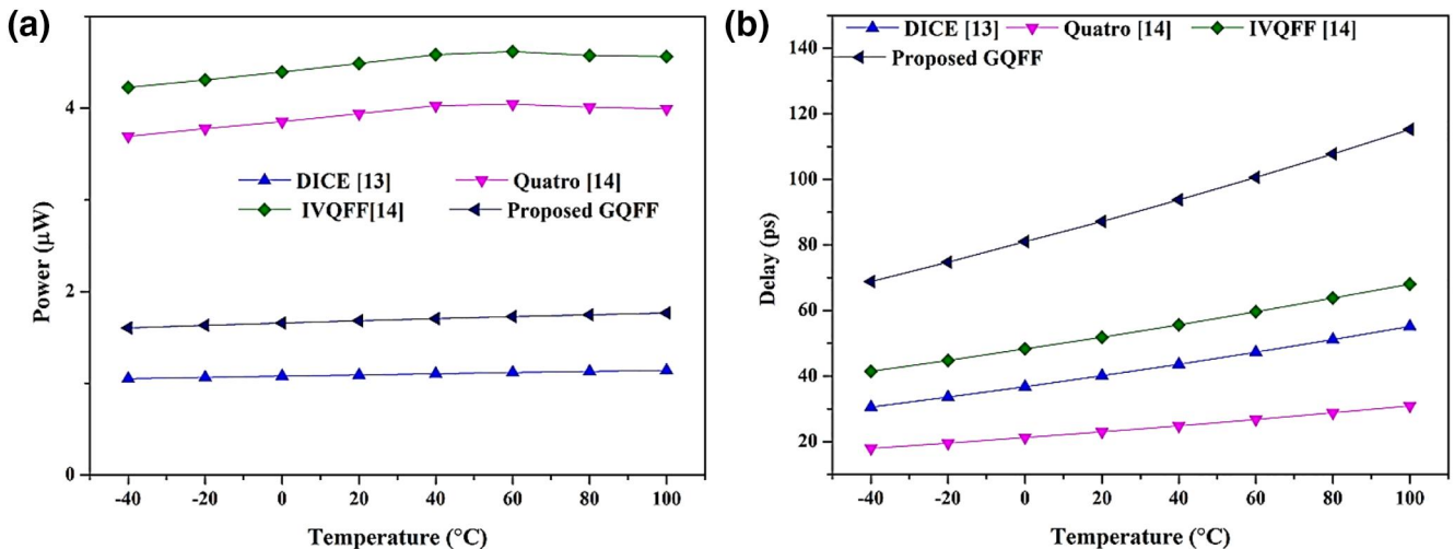
FIGURE 12 Temperature variation impact on (a) power dissipation and (b) Delay (CLK to Q). CLK, clock
