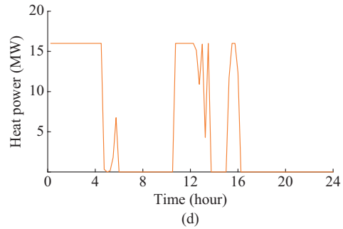
Fig. 11. Scheduling results with HSD and EB. (a) Wind power. (b) Photovoltaic. (c) Heat storage of HSD. (d) Heat power of EB.
