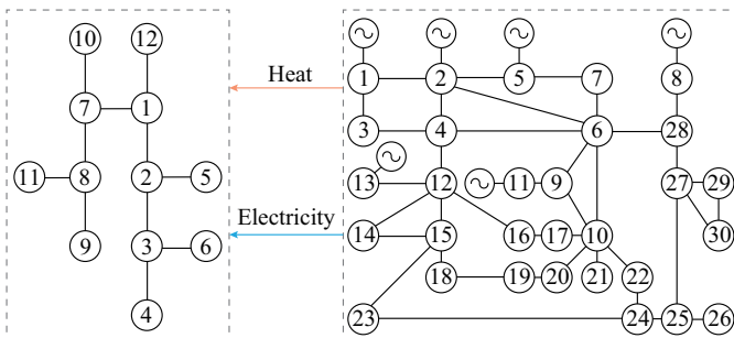
Fig. 16. Diagram of 30-bus and 12-node large system.
