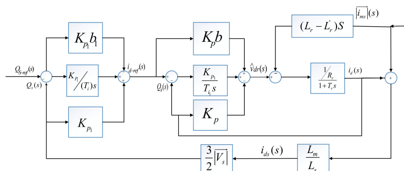
Figure 5. Control loop related to stator reactive power.
