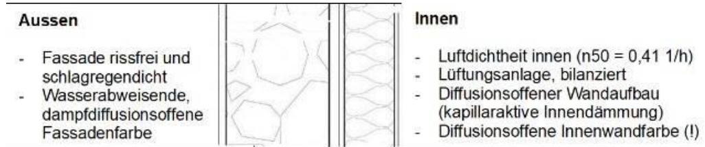
figure 3: cross section: concept of the internal insulation, ©Valentina Cari
