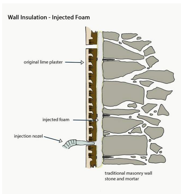
figure 86: Indicative diagram showing the foam being injected behind the lath and plaster lining © HES
