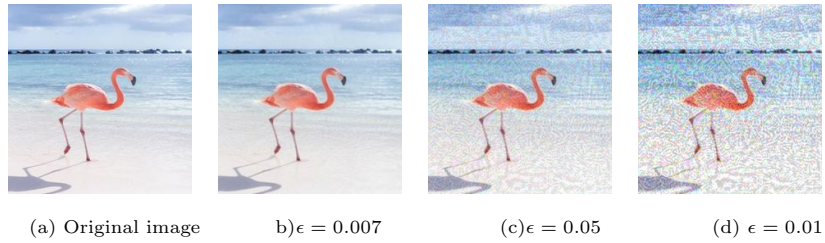
Figure 11: Example of a natural image 'Flamingo' in its original form and also with three different levels of FGSM noise, together with the corresponding predictions 'American egret', 'Nematode' and 'Nematode'.
