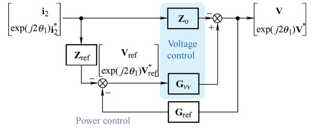
Fig. 2 Closed-loop \alpha\beta -frame model of grid-forming VSC [26]
