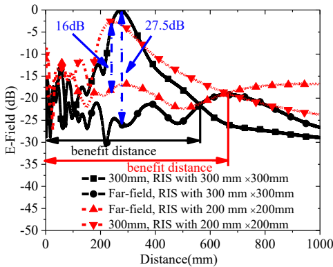
Fig. 13. The electric fields along the boresight direction for the RISs with dimensions of 200mm × 200mm and 300mm × 300mm.
