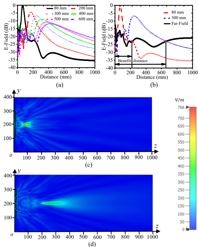
Fig. 4. Near-field focusing performance of a RIS. (a). The electric field along the boresight direction with the assigned focal distances of 80, 200, 300, 400, 500, 600mm. (b). The electric field along the boresight direction with the assigned focal distance of 80 and 300mm, and the referred far-field. (c). The electric-field distribution on the yo z -plane with the assigned focal distance of 80mm. (d). The electric-field distribution on the yo z -plane with the assigned focal distance of 300mm. (The units for y - and z -axis are millimeters in both Figs. (c) and (d)).
