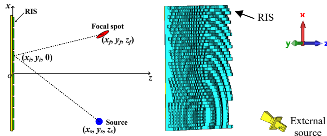
Fig. 3. (a). A simple diagram of a RIS illuminated with an external source to achieve a focal spot in the near-field region. (b). An example of the simulation model in CST software.
