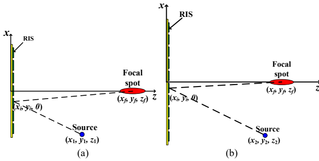
Fig. 12. Configurations of the RISs with different sizes. (a). 200mm × 200mm. (b). 300mm × 300mm.
