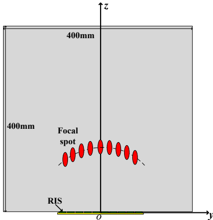
Fig. 5. The diagram of the scanning radiation beam/focal spot on the yo\text{-}z -plane.
