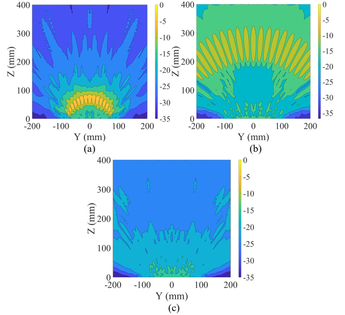
Fig. 6. The total scan patterns within the area of interest ( 400\text{mm} \times 400\text{mm} on the yo\text{-}z -plane) at 26GHz. (a). Near-field focusing RIS with an assigned focal distance of 80 mm. (b). Near-field focusing RIS with an assigned focal distance of 300mm. (c). Conventional far-field focusing RIS. (All values are normalized to the maximum electric-field amplitude of Fig. 6(a).)
