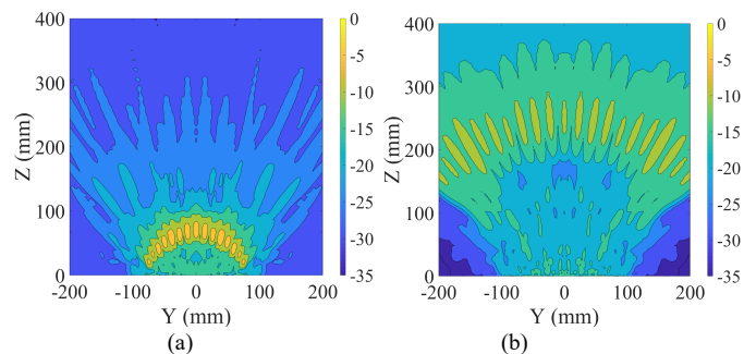
Fig. 10. The total scan patterns within an area of 400\text{mm} \times 400\text{mm} on the yo z-plane at 26GHz. (a). 1-bit near-field focusing RIS with an assigned focal distance of 80mm. (b). 1-bit near-field focusing RIS with an assigned focal distance of 300mm. (All values are all normalized to the maximum electric-field amplitude of Fig. 6(a).)
