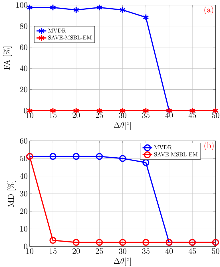
Fig. 10 Simulation results. a False alarm rate in low-reverberation environment. b Miss-detected rate in low-reverberation environment
