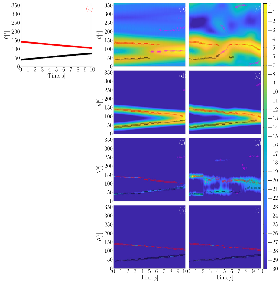
Fig. 9 Estimation results for the second virtual room setup. For the CBF, MVDR and SRP-PHAT methods, the estimation results are shown using the spatial spectrum of all frames. For the proposed SAVE-MSBL-EM method, the estimation results are shown using the weights \mathbf{w} of all frames. a The trajectories of two source. b Estimation result of CBF method in free field. c Estimation result of CBF method in low reverberation. d Estimation result of SRP-PHAT method in free field. e Estimation result of SRP-PHAT method in low reverberation. f Estimation result of MVDR method in free field. g Estimation result of MVDR method in low reverberation. h Estimation result of the proposed method in free field. i Estimation result of the proposed method in low reverberation
