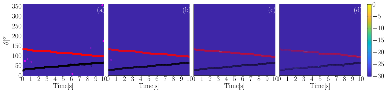
Fig. 11 The performance of the proposed method versus different number of snapshots L in a frame. a L = 1 . b L = 5 . c L = 10 . d L = 15
