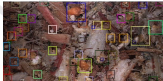
(c) SieveNet
