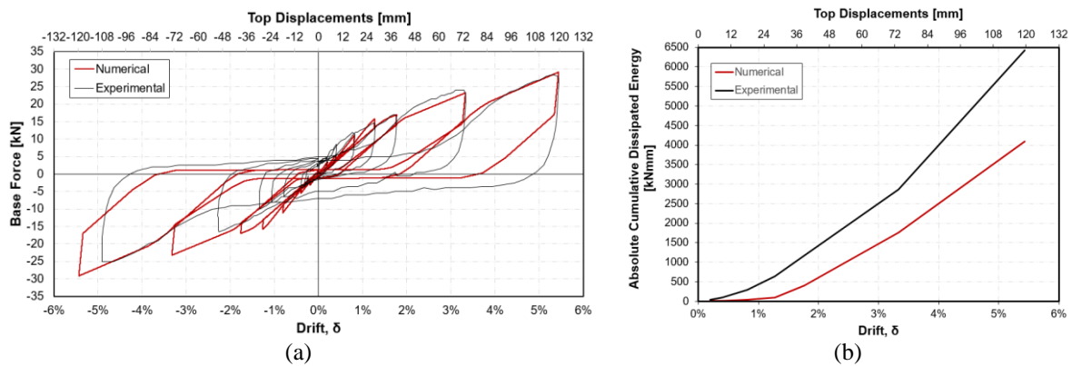
Figure 7: Experimental and numerical hysteretic curve (a) and absolute cumulative dissipated energy (b) [8]
