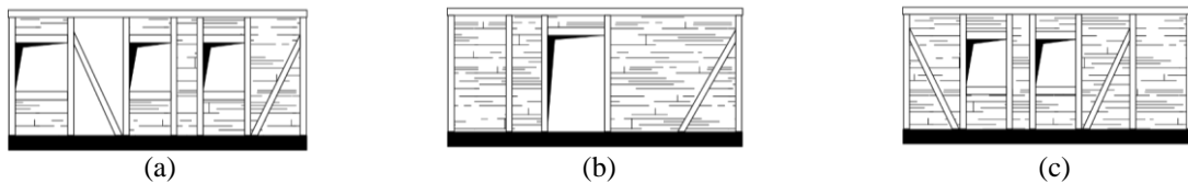
Figure 2: Elevation of TW1 (a), TW2 and TW3 (b), TW4 (c) wall [8]
