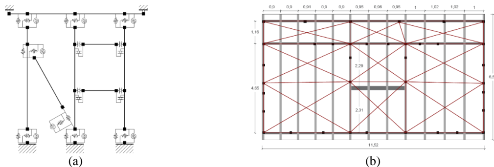
Figure 9: Structural scheme of walls (a) and floor (b)
