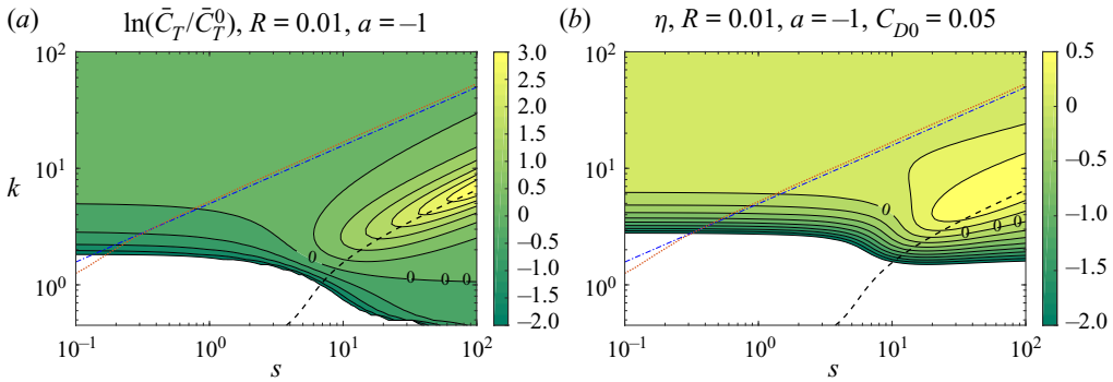
Figure 13. Thrust coefficient (a) and efficiency (b) as a function of frequency k and stiffness ratio S for a pitching motion about the leading edge ( a = -1 ) with R = 0.01 ( a_0 = 2^\circ and C_{D0} = 0.05 ). The lines marked with '0' in (a) indicate where the flexible foil has the same thrust as the equivalent rigid foil ( \bar{C}_T^0 ). Areas with negative thrust have been whited out in (a), while values less than -2 are whited out in (b). The dashed lines correspond to the first natural frequency of the system k_r that minimizes |F_2| , while the dashed-and-dotted line in (a) is k_{r0} given by (3.5). The dotted lines are the second natural frequency computed by Floryan & Rowley (2018) for this case (extracted from their figure 15).
