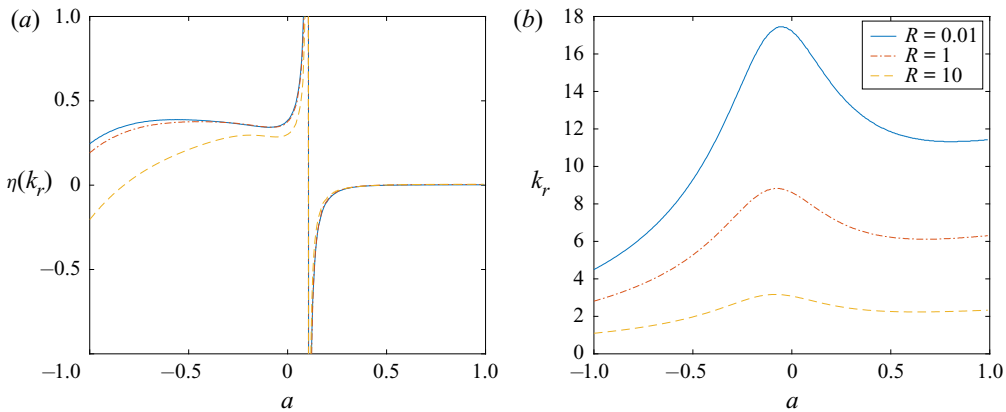
Figure 10. Efficiency at k = k_r as a function of the pivot point location ( a ) and the corresponding k_r ( b ) for S = 50 and three values of R , for a purely heaving motion with h_0 = 0.02 and C_{D0} = 0.05 .
