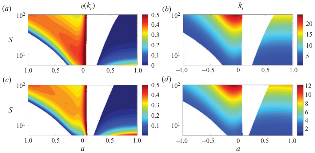
Figure 11. Efficiency at k = k_r(a, c) and the corresponding k_r(b, d) in the stiffness–pivot point location plane for a purely heaving motion with h_0 = 0.02 and C_{D0} = 0.05 , for R = 0.01 (a, b) and R = 1 (c, d). Areas with negative efficiency have been whited out.
