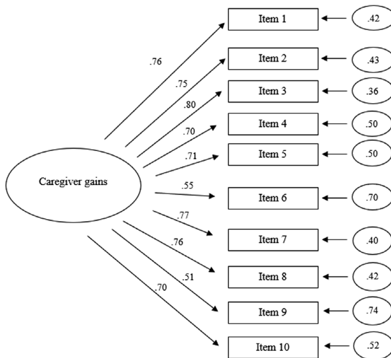
Figure 1. Single-factor model for the GAIN, with standardized parameter values. Note. N = 113. \chi^2 = chi-squared statistic, \chi^{2SB} = Satorra-Bentler chi-squared, df = degrees of freedom, CFI = comparative fit index, NNFI = non-normed fit index, RMSEA = root mean square error of approximation, with a 90% confidence interval.
