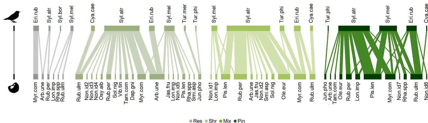
Fig. 5. Seed dispersal networks of the four sampling areas. Seed-dispersing birds are shown in the upper level of the network and dispersed plant species in the lower level. All networks are shown in the same scale. A single interaction is represented by the line thickness of the example on the left side of the image. Bird species abbreviations: Cya.cae (blue tit Cyanistes caeruleus ), Eri.rub (European robin Erithacus rubecula ), Syl.atr (Eurasian blackcap Sylvia atricapilla ), Syl.bor (garden warbler Sylvia borin ), Syl.mel (Sardinian warbler Sylvia melanocephala ), Tur.mer (blackbird Turdus merula ), Tur.phi (song Thrush Turdus philomelos ). Res (restored quarry area), Shr (natural shrubland), Mix (mixed open forest) and Pin (Aleppo pine forest). For plant species abbreviations: Table S9, Supporting information. (For interpretation of the references to colour in this figure legend, the reader is referred to the Web version of this article.)
