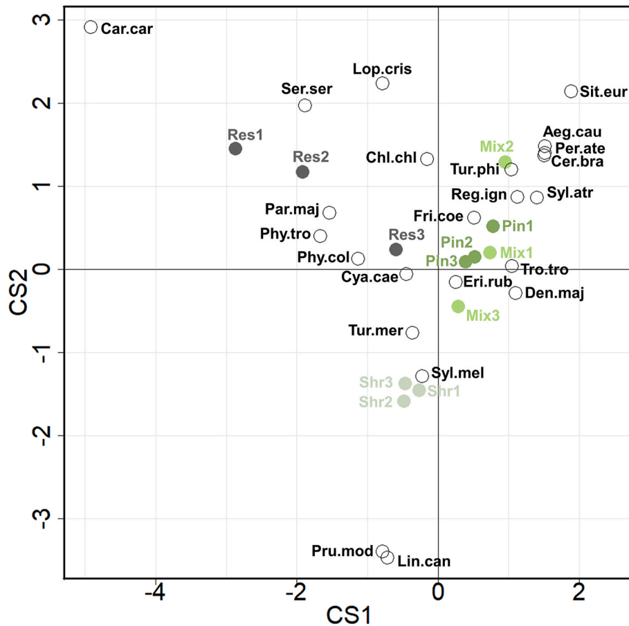
Fig. 3. Correspondence analysis of bird communities: species scores are represented as empty circles and plot scores as filled circles. Res (restored quarry area), Shr (natural shrubland), Mix (mixed open forest) and Pin (Aleppo pine forest). For species abbreviations: Table S3, Supporting information.
