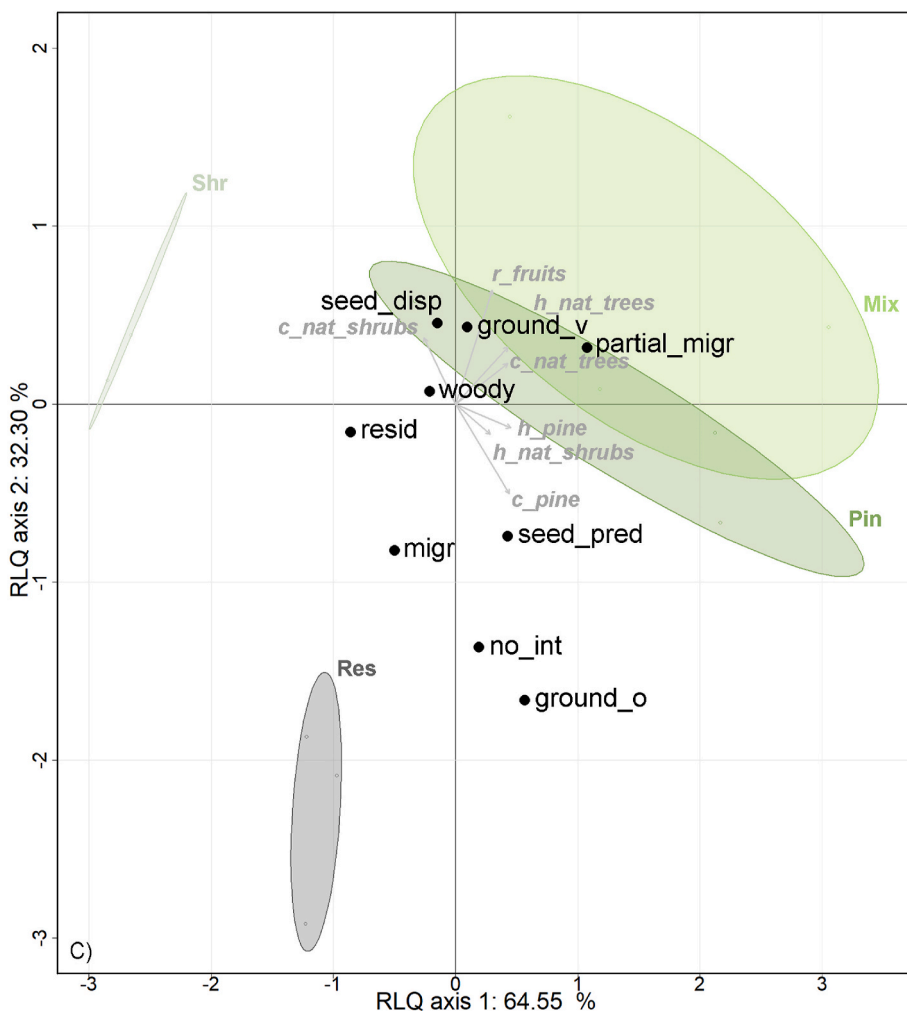
Fig. 4. RLQ showing vegetation and trait vectors. Ellipses represent 50 % of the total variation of vegetation scores per area. Res (restored quarry area), Shr (natural shrubland), Mix (mixed open forest) and Pin (Aleppo pine forest). For vegetation and trait abbreviations: Tables S1 and S2, Supporting information.
