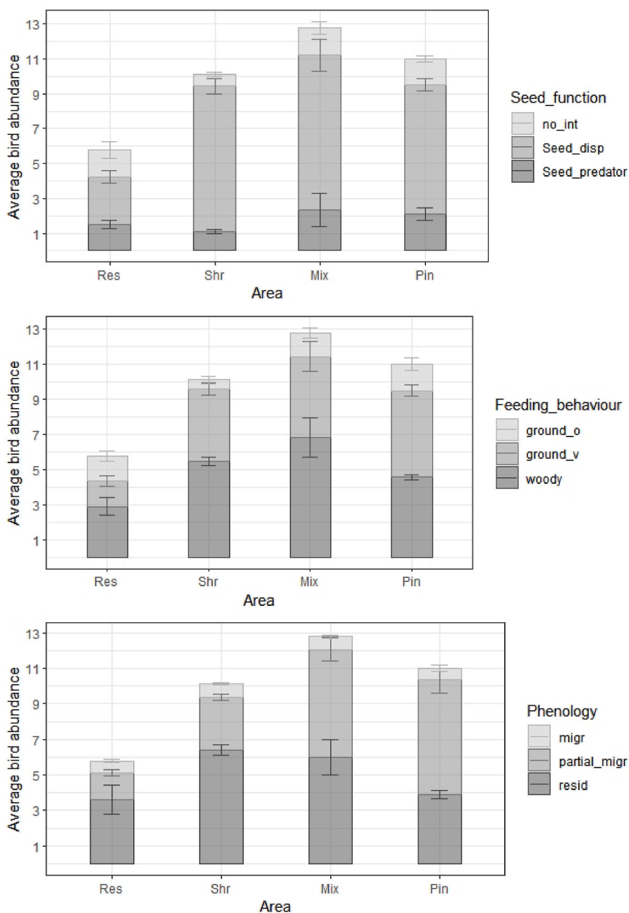
Fig. 2. Bird abundances in each area partialled out by ecological function towards seeds of fleshy fruited species, feeding behaviour and phenology (bars). Whiskers represent ± standard deviation. For traits abbreviations see Table S2, Supporting information. Res (restored quarry area), Shr (natural shrubland), Mix (mixed open forest) and Pin (Aleppo pine forest).
