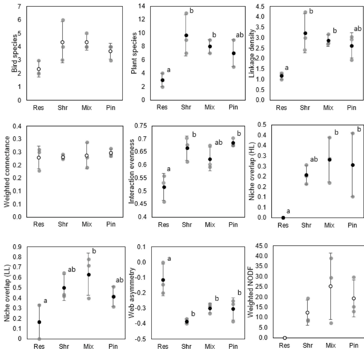
Fig. 6. Mean and standard deviations of network metrics for each area. Black filled dots represent average values of the metrics with significant differences between areas. Grey dots represent metric values per plot. Res (restored quarry area), Shr (natural shrubland), Mix (mixed open forest) and Pin (Aleppo pine forest).
