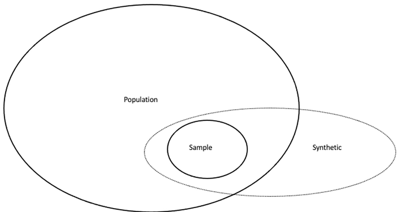
Fig 1. Relationship between population, sample and synthetic data [10].
