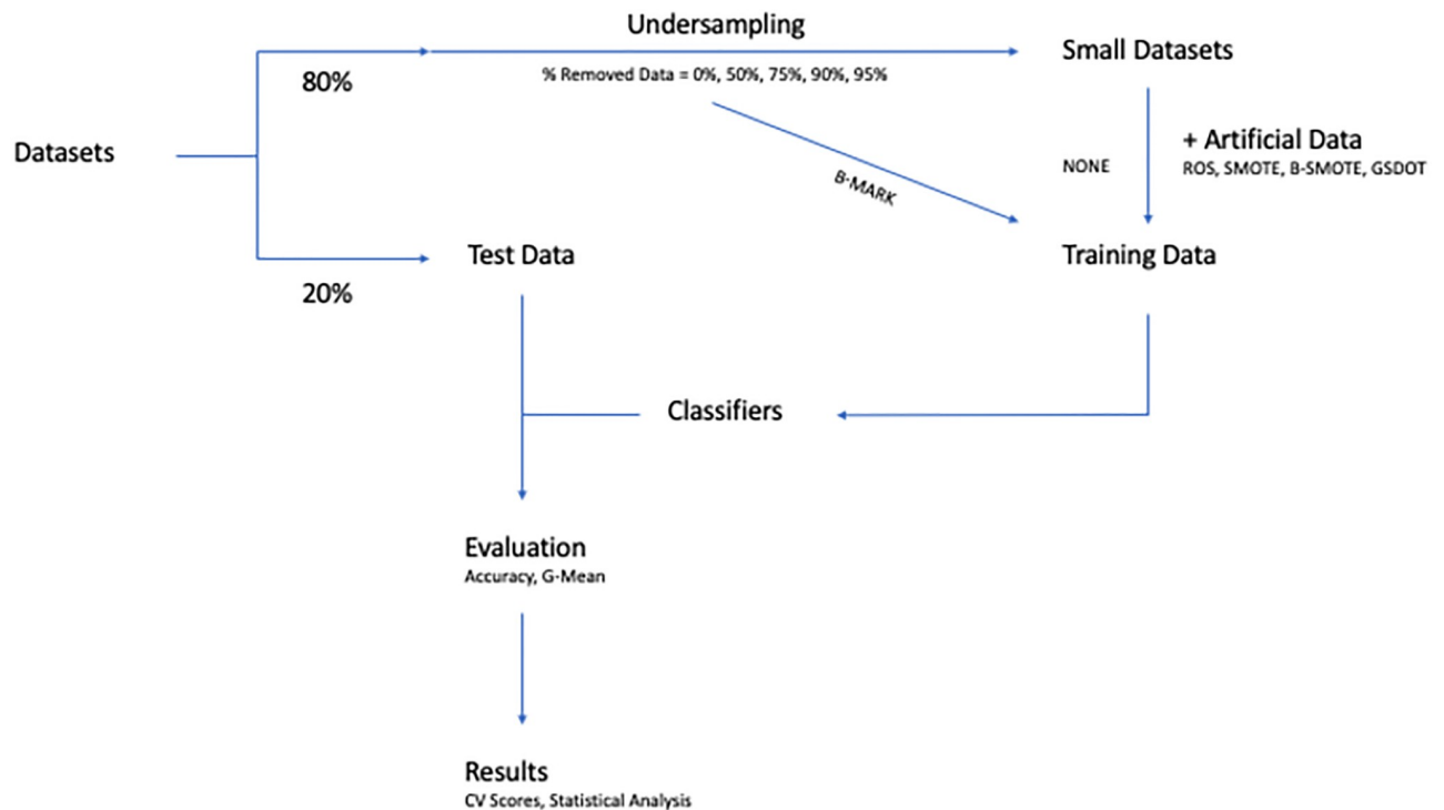
Fig 3. Visualization of the experimental procedure.
