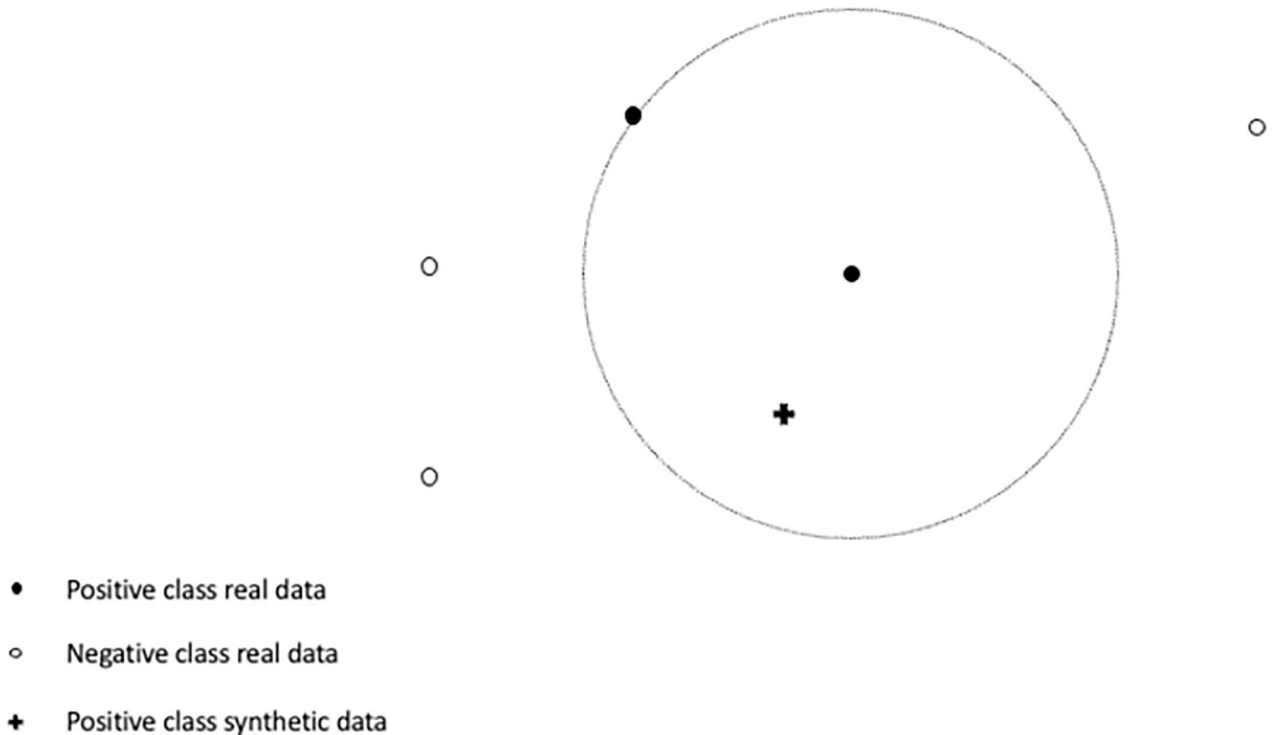
Fig 2. The GSDOT data generation mechanism when positive class samples are generated. The process is repeated for the negative class.
