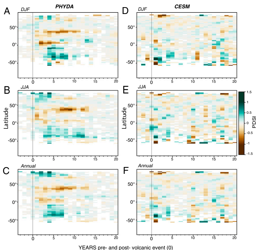
Fig. 2. The Hovmöller diagram showing the weighted zonal mean response to TVEP or TVE in different seasons (A–C) using PHYDA and (D–F) CESM ensemble member 10, respectively. Values that do not satisfy the significance threshold ( P < 0.05 ) are excluded. The vertical black line indicates the onset of the volcanic event. Greenland and Antarctica are not included.
