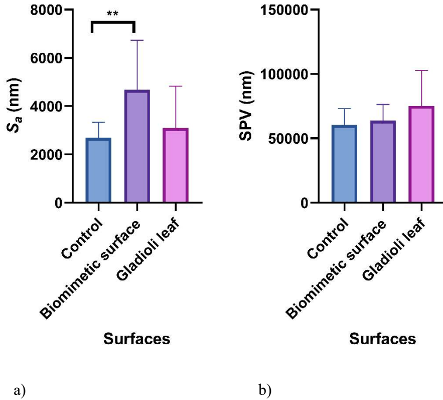
Figure 2. Surface roughness parameters ( S_a (a) and S_{pv} (b)) of the unmodified wax surface, biomimetic wax surface, and original Gladioli leaf obtained from the optical profilometry images. The means + standard deviations are presented and asterisks denote significance (** p \leq 0.01 ).
