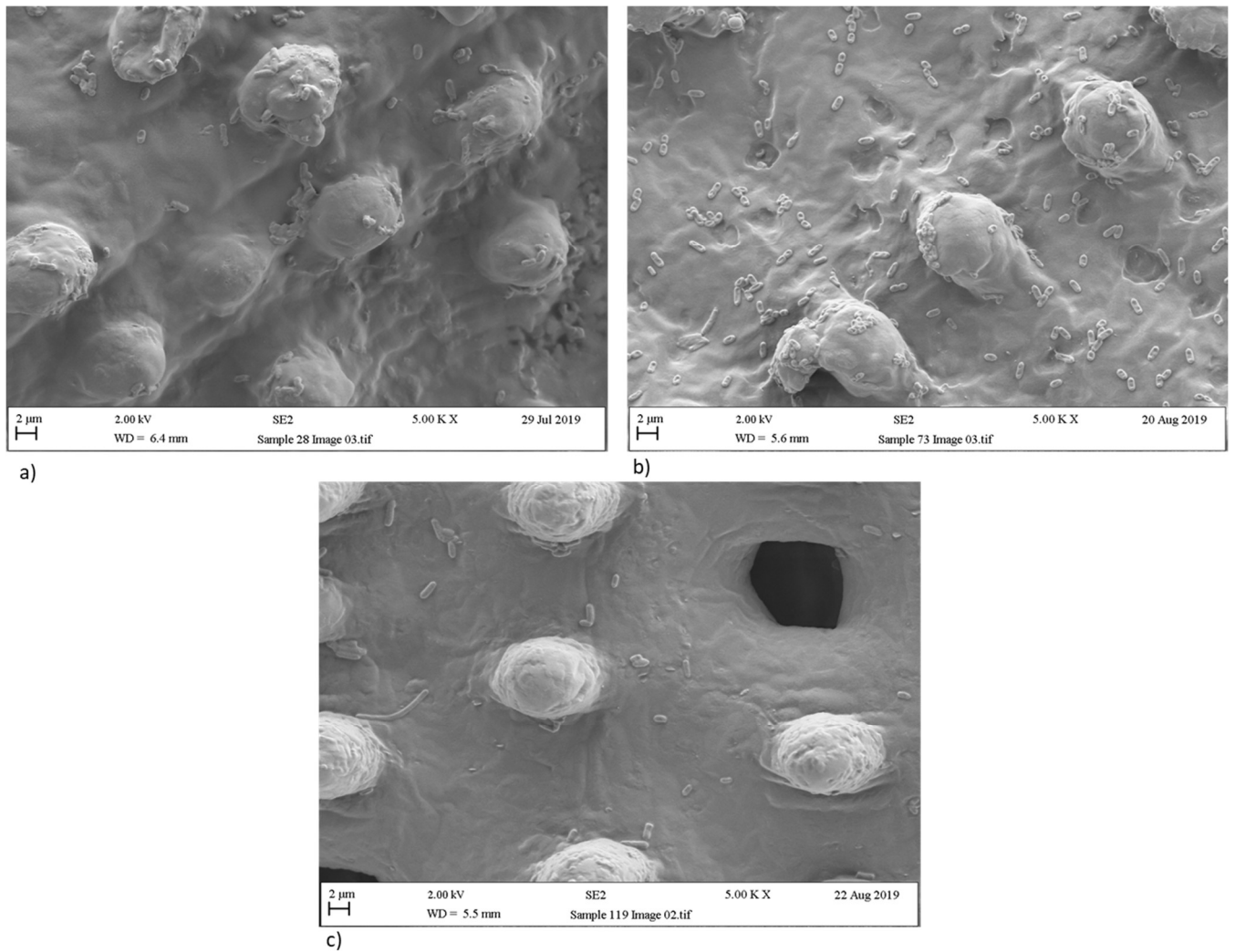
Figure 6. Scanning electron micrographs of bacteria retained on biomimetic surfaces: a) E. coli in monoculture, b) L. monocytogenes in monoculture, and c) E. coli and L. monocytogenes in co-culture.
