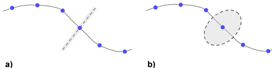
Fig. 9 Models of point positional uncertainty: a random variable associated to a displacement in the direction defined by the local surface normal, b full three-dimensional probability ellipsoid (tri-variate random variable) associated to each point (from Catalucci and Senin [120])
