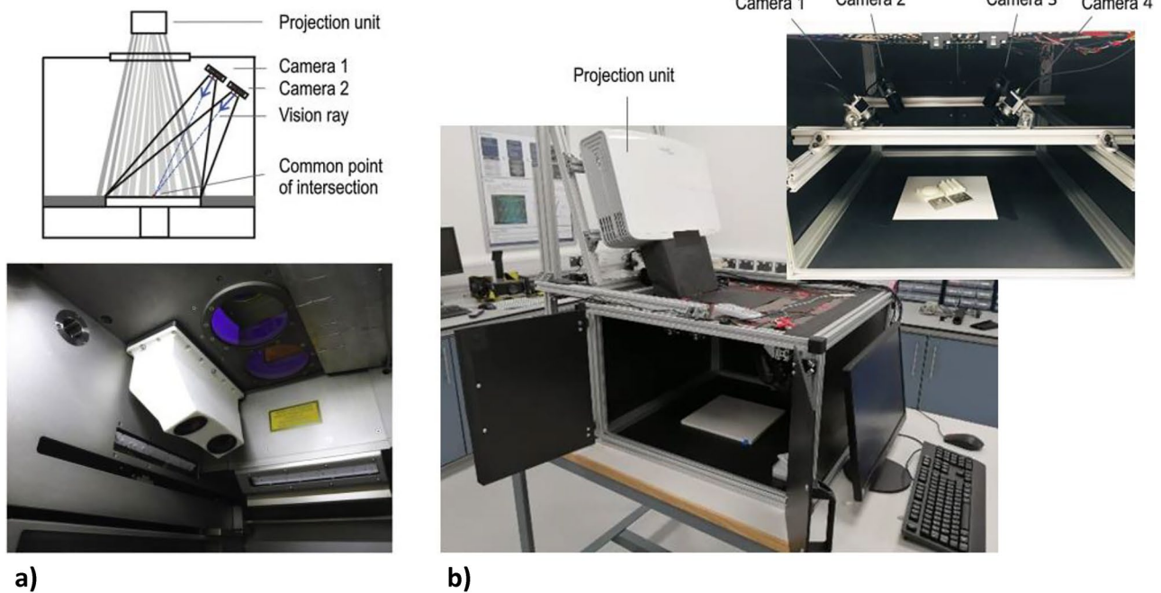
Fig. 5 Example setups of multi-view configurations for the acquisition of topographical information of surface texture: a two-camera fringe projection system installed inside a laser beam melting (LBM)
