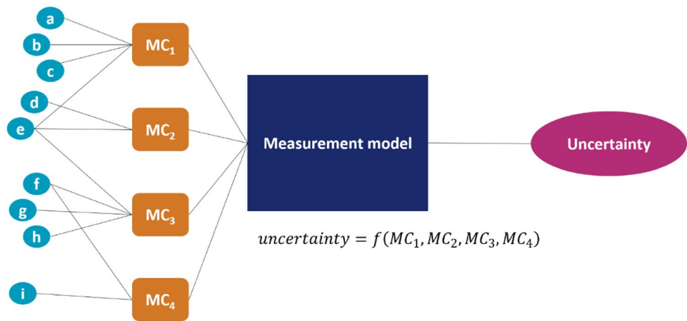
Fig. 10 Illustration of the metrological characteristics framework to estimate measurement uncertainty. (a) to (i) are influence quantities and MC1 to MC4 are metrological characteristics (from Leach et al. [149])
