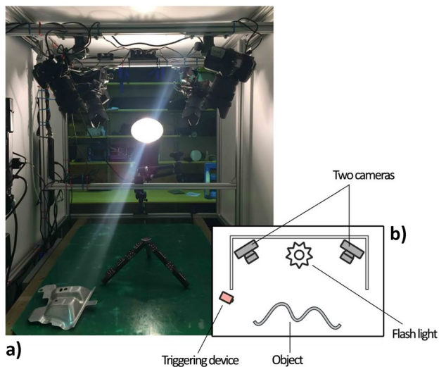
Fig. 6 Photogrammetry for in-line inspection. The setup proposed by Bergstrom et al. [84] consists of two cameras, a flash light, and a triggering device. The sensor is placed on one end of the conveyor belt: a picture of the setup; b schematic of the design
