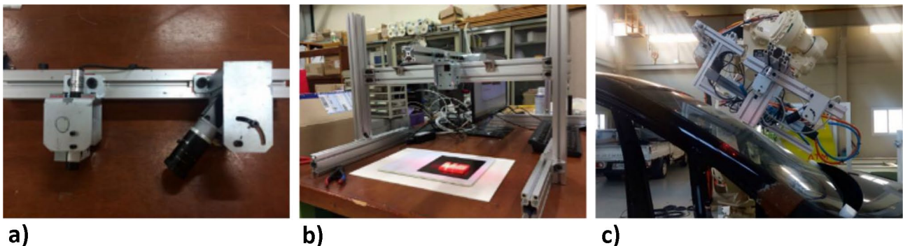
Fig. 3 Measurement of gap/flush in assembly of automotive vehicles: setup developed by Tran and Ha [34]. a Camera-laser module (high-resolution camera and a multi-line laser-based sensor), b view of the
