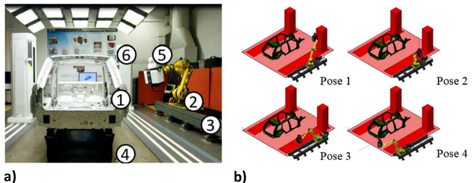
Fig. 2 In-line dimensional inspections using laser radar: industrial demonstrator developed by Kiraci et al. [32]: a experimental setup (1, work-piece; 2, robot; 3, trail; 4, tooling balls; 5, laser radar sensor; 6, tactile coordinate measuring system); b the four positions of the trail
