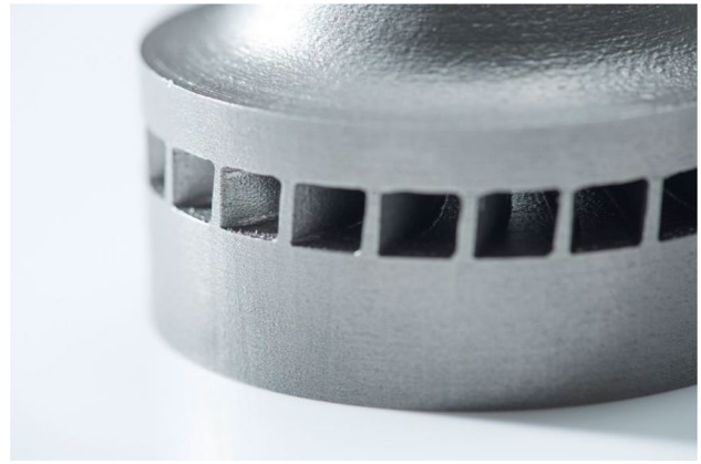
Fig. 7 Example complex AM part containing features that are problematic for optical measurement systems, because of a lack of line-of-sight resulting from occlusion
