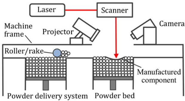
Fig. 4 Schematic example of in-process fringe projection setup in laser powder bed fusion (LPBF) (from Gao et al. [27])
