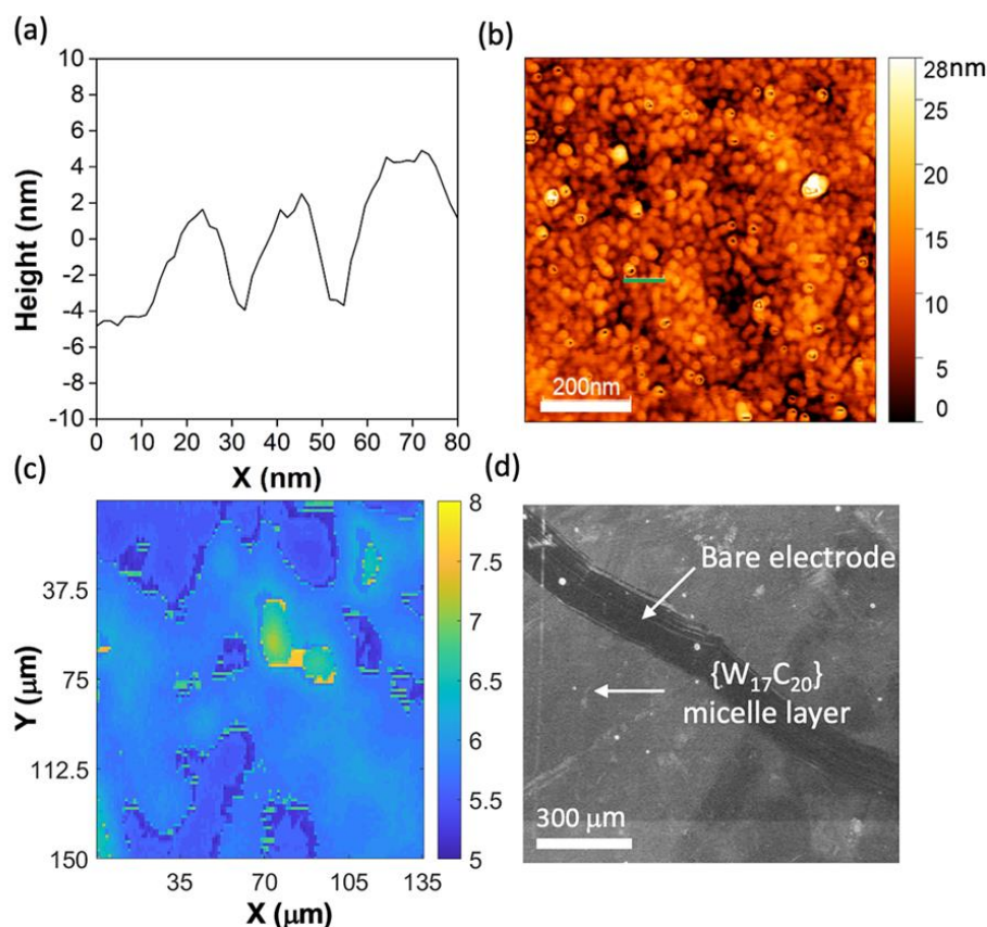
Figure 3. a) \{W_{17}C_{20}\}@GC electrode height trace plot of section highlighted (green) in panel b, (peak full width half maxima = 12.1 nm); b) AFM plot of \{W_{17}C_{20}\}@GC electrode; c) ellipsometry map of the prepared GC square electrode post CV, displaying regions of deposition from 5–8 nm thickness; d) SEM image displaying areas of deposition (light grey) and an area of bare electrode that has been (inadvertently) mechanically abraded (dark grey).
