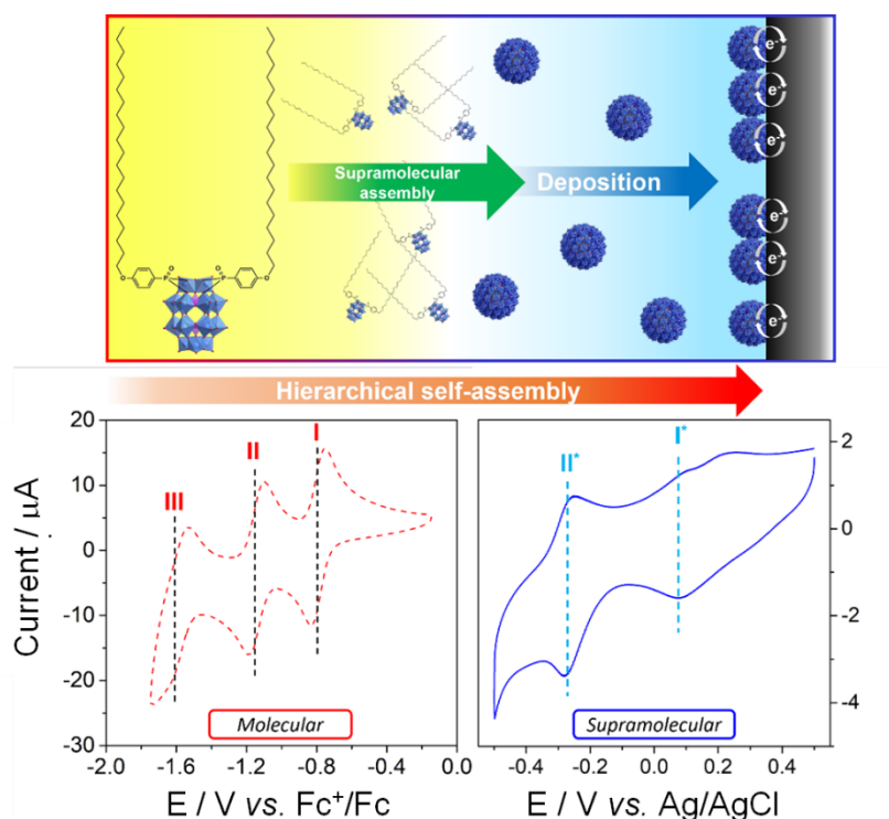
Figure 1. A schematic illustrating the hierarchical supramolecular assembly of redox-active \{\text{W}_{17}\text{C}_{20}\} in aqueous solutions onto glassy carbon, and CV plots of (red) 1.4 mM \{\text{W}_{17}\text{C}_{20}\} in DMF (i.e. the molecular system) with 0.1 M [\text{TBA}][\text{PF}_6] , and; (blue) 1.4 mM \{\text{W}_{17}\text{C}_{20}\} in 0.1 M \text{H}_2\text{SO}_4 (i.e. the surface-bound system).
