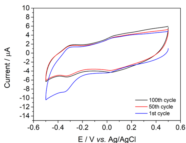
Figure 2. A cyclic voltammogram of \{W_{17}C_{20}\} deposited on a GC electrode displaying cycles 1 (blue), 50 (red) and 100 (black) in 0.1 M H_2SO_4 supporting electrolyte.
