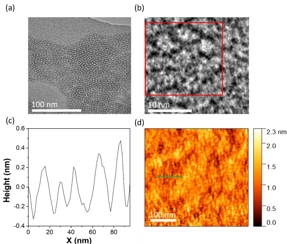
Figure 4. a) TEM image of micelle packing nanopattern assembled by drop casting 1.4 mM \{W_{17}C_{20}\} on to GO TEM grid; b) high magnification image, highlighting the packing of the micelles on GO (focused in red box); c) height trace plot from the area highlighted by the green line in panel d (peak half width full maxima = 5.5 nm), and; d) atomic force microscopic surface analysis of the micelle packing on a GO TEM grid.
