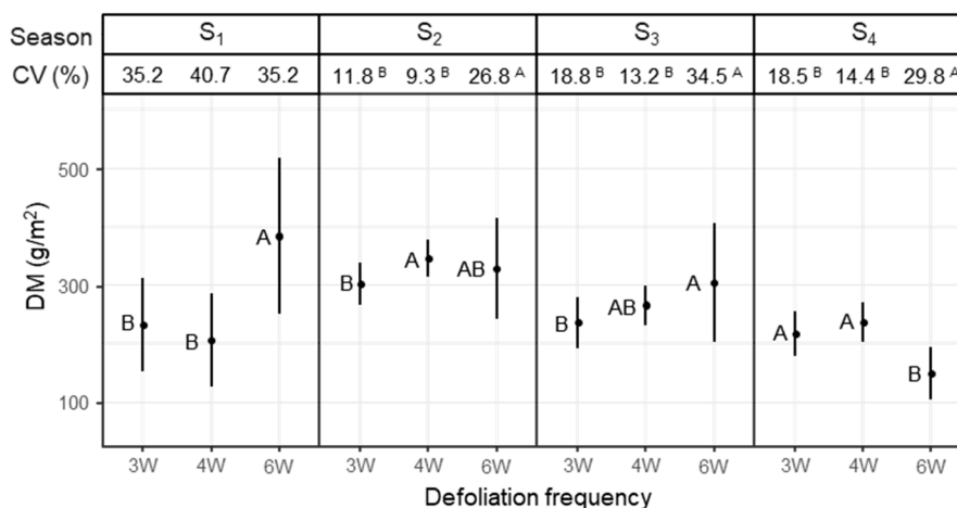
Figure 4. Effect of defoliation frequency on seasonal DM yields (mean \pm SD) and their inter-annual coefficient of variation (CV). Capitals indicate significant differences of DM yields or CVs between defoliation frequencies (3W, three-weekly simulated grazing; 4W, four-weekly simulated grazing; 6W, cutting for conservation) within seasons.
