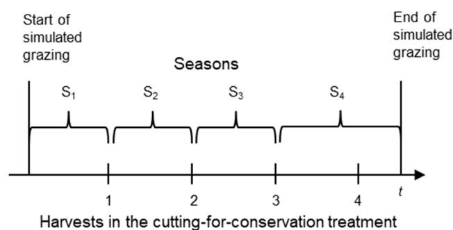
Figure 1. Annual fragmentation of the growing period into seasons ( S_1 – S_4 ) in accordance to the cutting dates in the cutting-for-conservation system.
