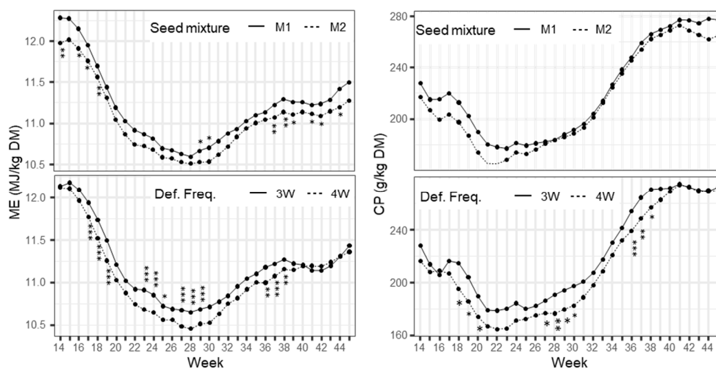
Figure 3. Average ME and CP contents during the growing season. Asterisks indicate the level of significance of differences between seed mixtures (upper graphs) and defoliation frequencies (lower graphs).
