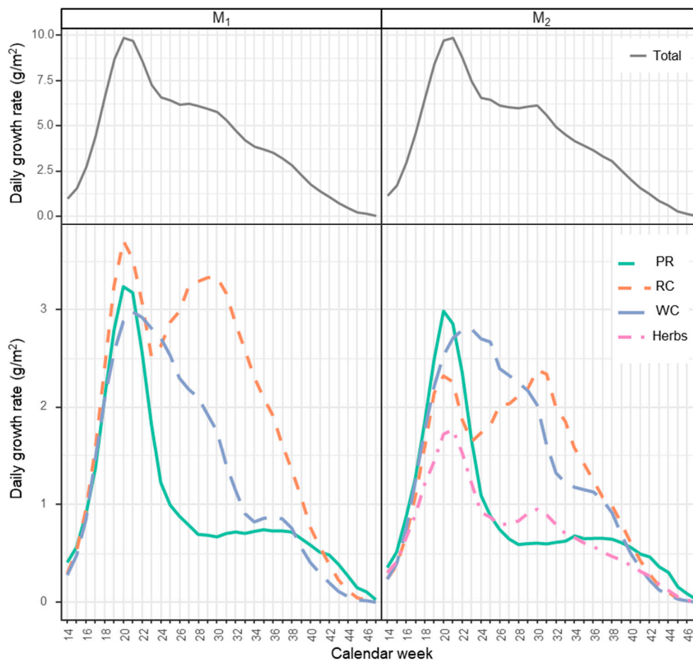
Figure 2. Daily growth rates of both seed mixtures averaged across defoliation frequencies (3W and 4W). The upper curves represent the total herbage growth, the lower curves the growth of PR, RC, WC, and the group of forage herbs.
