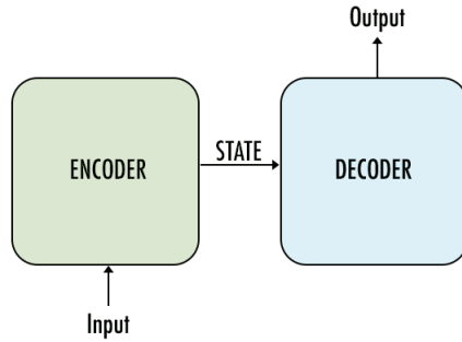
FIGURE 1.1 – Architecture encodeur-decodeur
