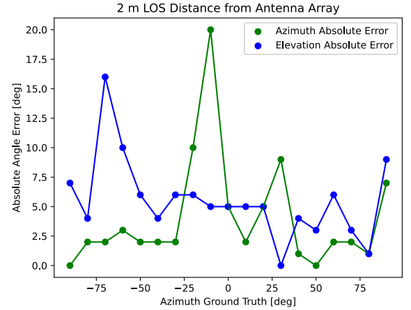
FIGURE 12. AoA estimation absolute azimuth and elevation error at 2 m distance between the mobile device and antenna array in LoS, using Nordic Semiconductor kit.
