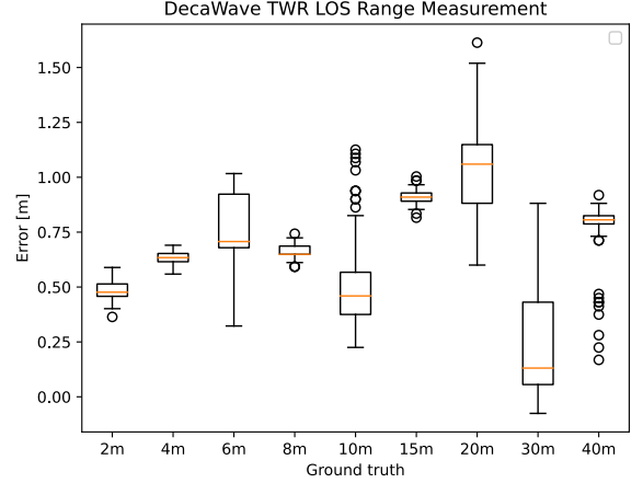
FIGURE 15. Box plot of TWR LoS distance measurement error between the two DWM1001-DEV.
