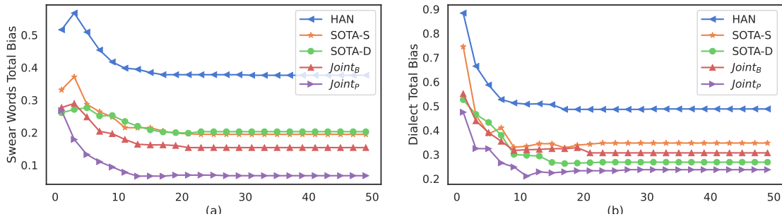
Figure 3: Instagram: The total biases (FPED + FNED) w.r.t. swear words and dialect. The x -axis denotes the number of comments ( t ) the agent has observed. SOTA-D in (a) shows the total bias w.r.t. Swear Words in the Dialect-debiased SOTA.
