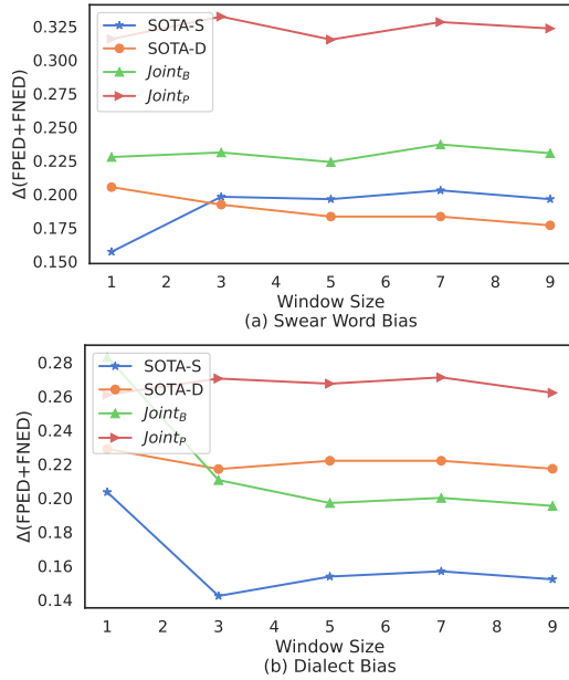
Figure 6: Instagram : \Delta(\text{FPED} + \text{FNED}) w.r.t. swear words and dialect biases for different window sizes. For example, \Delta(\text{FPED} + \text{FNED}) of SOTA-S is the difference between the total bias of SOTA-S and that of HAN. A larger value of \Delta indicates a greater reduction in bias.
