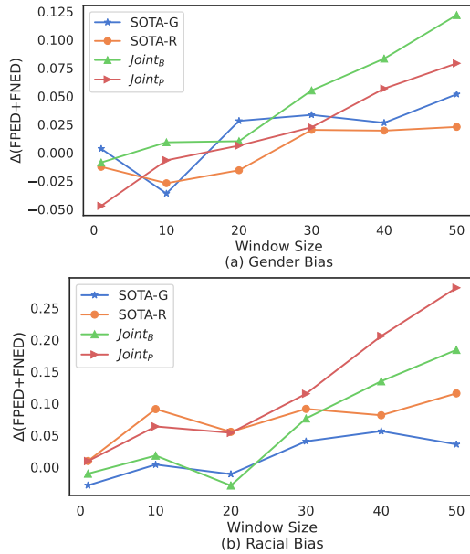
Figure 7: Jigsaw : \Delta(\text{FPED} + \text{FNED}) of racial and gender biases for different window sizes. For example, \Delta(\text{FPED} + \text{FNED}) of SOTA-G is the difference between the total bias of SOTA-G and that of HAN. A larger value of \Delta indicates a greater reduction in bias.
