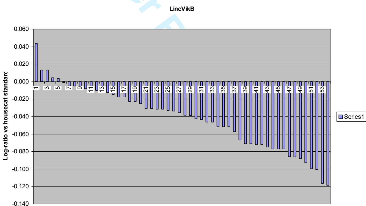
Fig 04. Log-ratio length and breadth distributions for Lincoln 10th to early 11th century cats.
