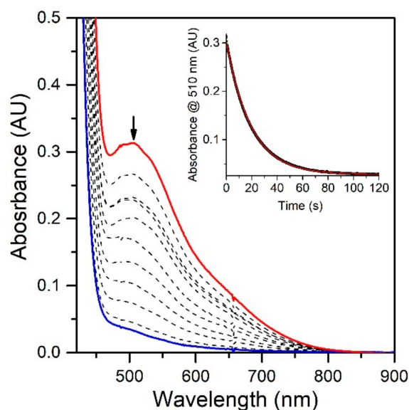
Figure 5. Reactions of 1.25 mM [\text{Mn}^{\text{III}}(\text{OH})(^6\text{Me dpaq})](\text{OTf}) with 10 equiv. TEMPOH at -35\text{ }^\circ\text{C} in MeCN (initial and final spectra are the red and blue traces, respectively). Inset: The decay of the 510 nm band over time (black trace) and fit to pseudo-first-order kinetic model (red trace).
