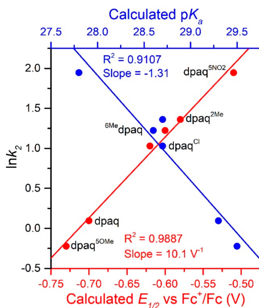
Figure 8. A plot of \ln k_2 vs. calculate E_{1/2} vs. Fc^+/Fc (V) and pK_a .
