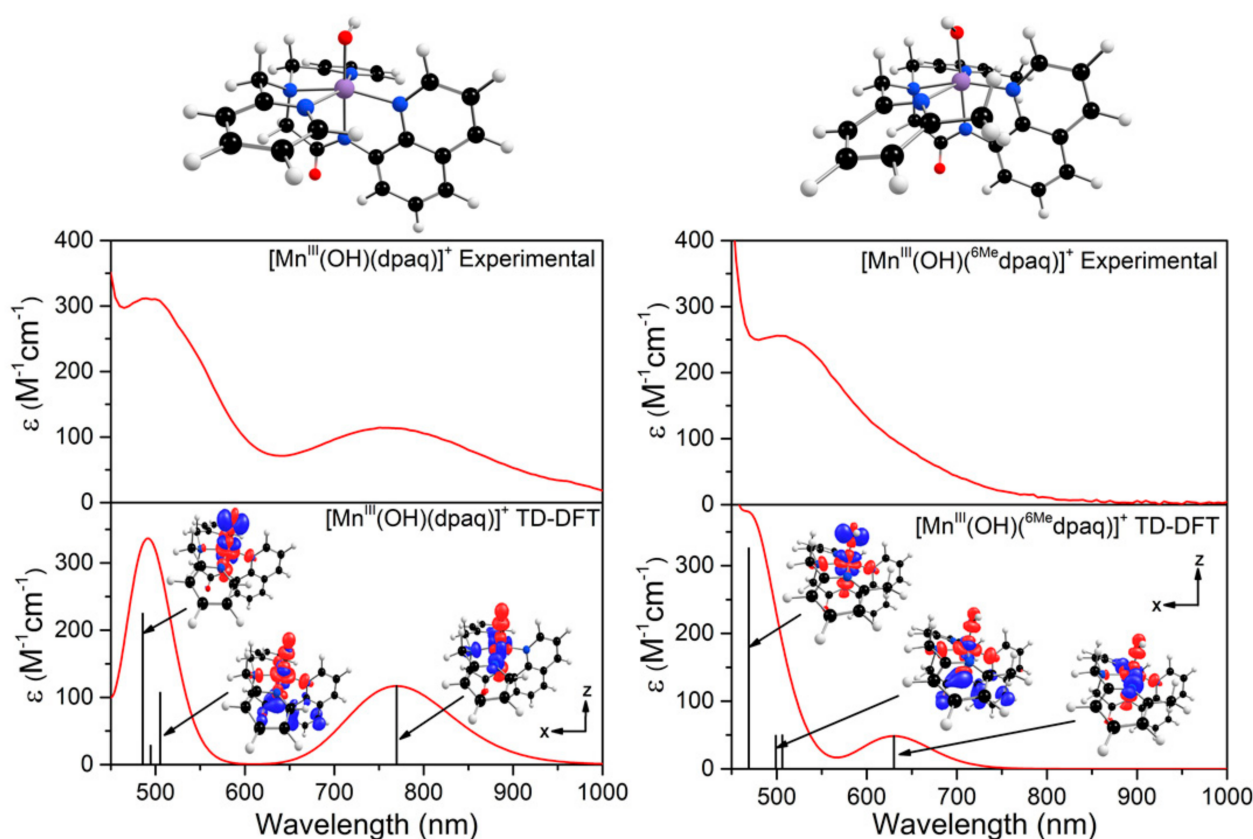
Figure 4. TD-DFT-computed electronic absorption spectra for [\text{Mn}^{\text{III}}(\text{OH})(\text{dpaq})]^+ (left) and [\text{Mn}^{\text{III}}(\text{OH})(^6\text{Me dpaq})]^+ (right). The sticks indicate electronic transitions; EDDMs of selected transitions are included as an inset. Red and blue colors in the EDDMs denote gain and loss of electron density, respectively. The DFT-computed structures of the \text{Mn}^{\text{III}} -hydroxo complexes are shown above the absorption spectra.
