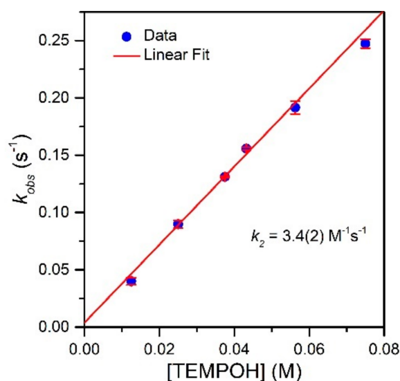
Figure 6. Pseudo-first-order rate constants k_{\text{obs}} ( \text{s}^{-1} ) as a function of TEMPOH concentration for a 1.25 mM solution of [\text{Mn}^{\text{III}}(\text{OH})(^6\text{Me dpaq})](\text{OTf}) in MeCN at -35\text{ }^\circ\text{C} . The second-order rate constant ( k_2 ) was calculated from the slope of the linear fit.
