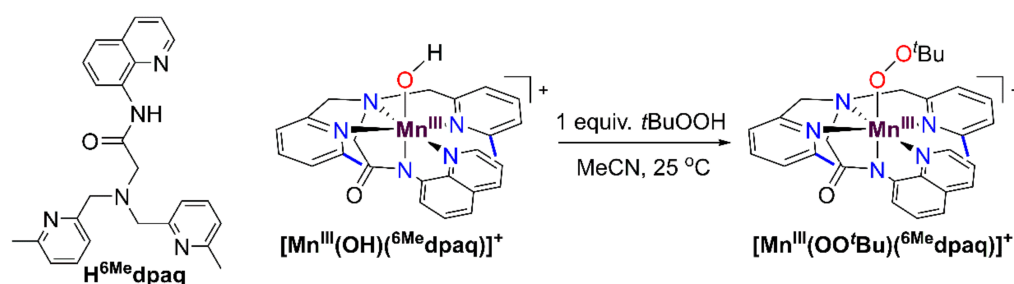
Scheme 2. Reaction of the \text{Mn}^{\text{III}} -hydroxo complex [\text{Mn}^{\text{III}}(\text{OH})(^6\text{Me dpaq})]^+ with t\text{BuOOH} to generate the \text{Mn}^{\text{III}} -alkylperoxy complex [\text{Mn}^{\text{III}}(\text{OO}^t\text{Bu})(^6\text{Me dpaq})]^+ . The structure of the protonated \text{Hdpaq}^{6\text{Me}} ligand is shown on the far left.
