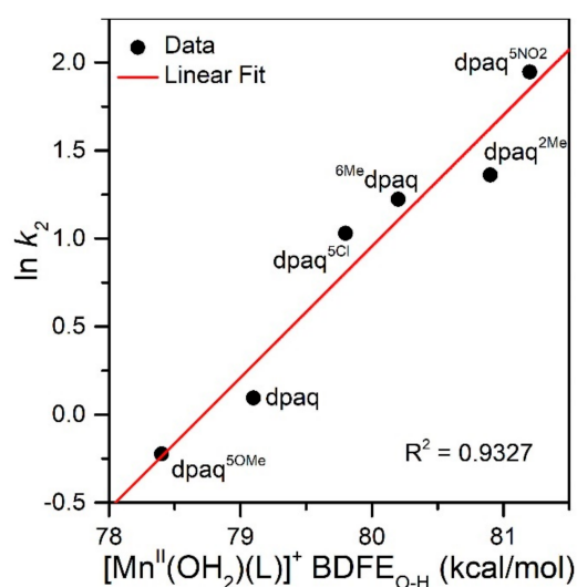
Figure 7. A plot of \ln k_2 vs. Mn II -aqua O–H BDFE (kcal/mol).
