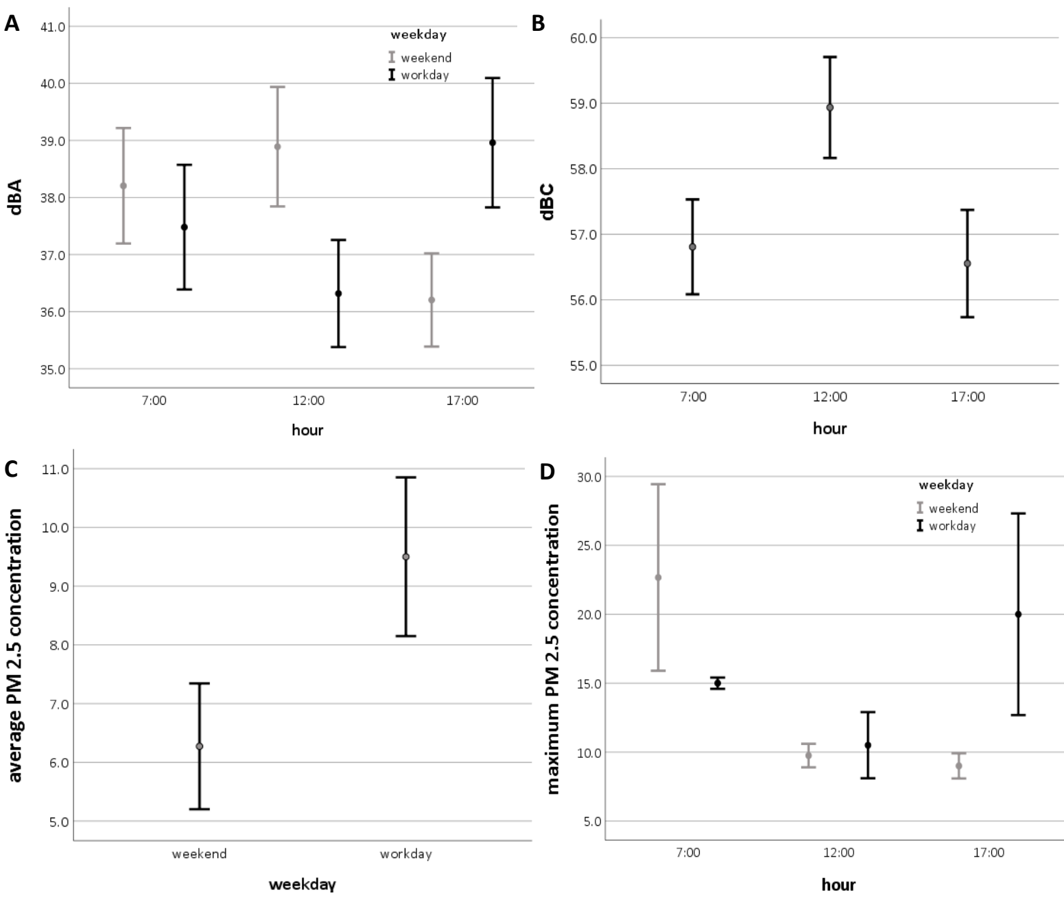
Fig. S3 Anthropogenic disturbance components in the study sites. Graphs show raw data means \pm SE. Noise pollution: A) mid-range noise (dBA); B) impulsive noise (dBC). Air pollution: C) average and D) maximum concentration of PM 2.5.
