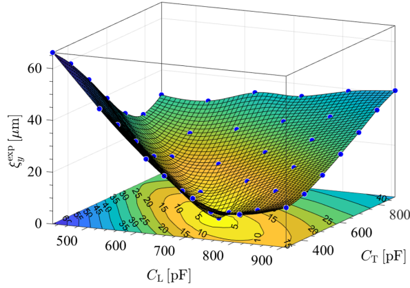
FIG. 6. Measured amplitudes of beam oscillations \xi_y^{\text{exp}} at BMP 17, plotted on a grid as a function of the variable capacitor values C_L and C_T . To avoid crowding up the map, the error bars of the data points were omitted, these are shown in Fig. 13 instead. The parameters of the matching point are given in Eq. (19).
